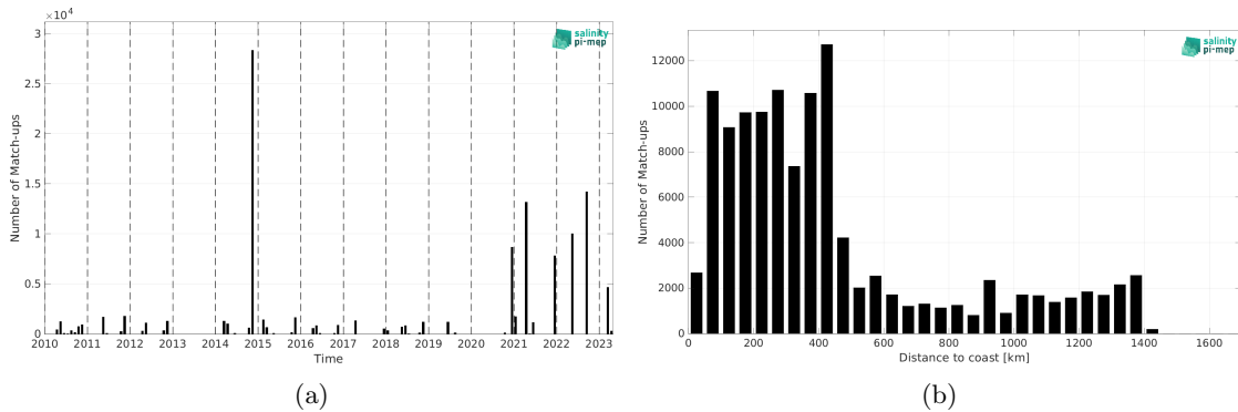
Figure 2: Number of match-ups between TSG (Polarstern) and SMOS SSS L3 v335 - Monthly - 25 km (CATDS-CPDC) SSS as a function of time (a) and as function of the distance to coast (b) over the North Atlantic Ocean Pi-MEP region and for the full satellite product period.
