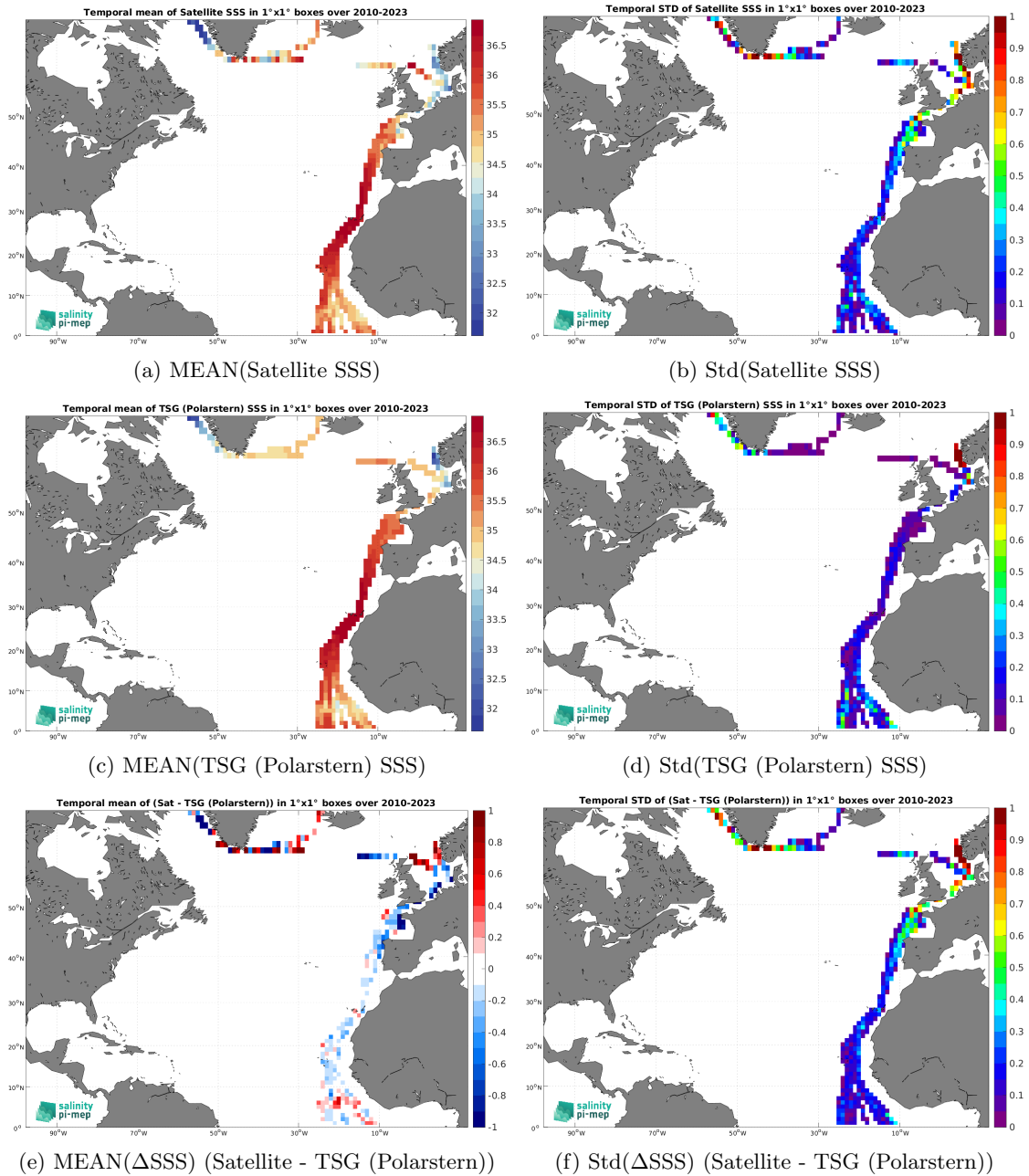
Figure 7: Temporal mean (left) and Std (right) of SSS from SMOS SSS L3 v335 - Monthly - 25 km (CATDS-CPDC) (top), TSG (Polarstern) (middle), and of \Delta SSS (Satellite - TSG (Polarstern)). Only match-up pairs are used to generate these maps.
