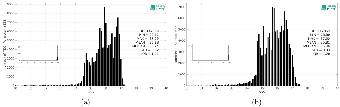
Figure 3: Histograms of SSS from TSG (Polarstern) (a) and SMOS SSS L3 v335 - Monthly - 25 km (CATDS-CPDC) (b) considering all match-up pairs per bins of 0.1 over the North Atlantic Ocean Pi-MEP region and for the full satellite product period.
