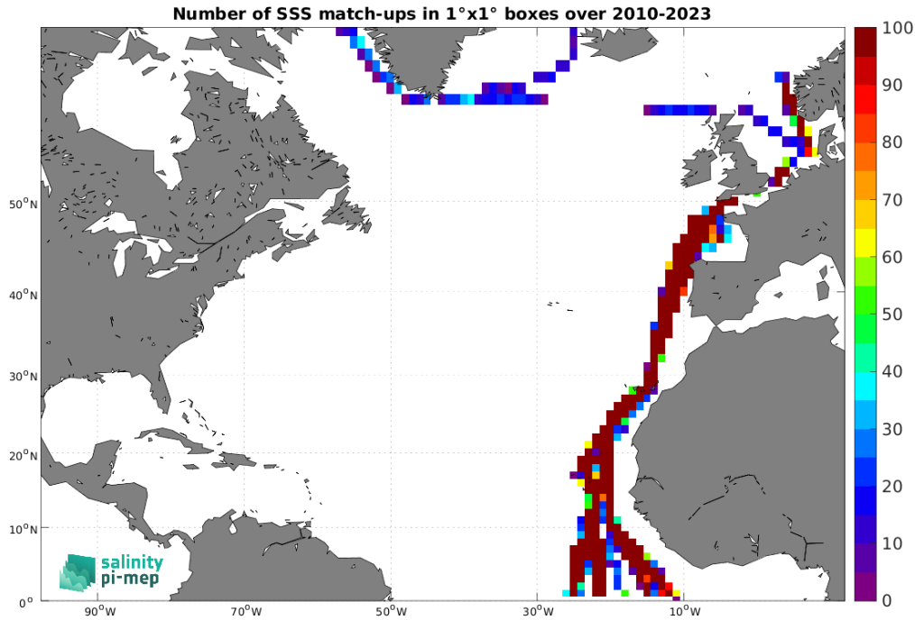
Figure 5: Number of SSS match-ups between TSG (Polarstern) SSS and the SMOS SSS L3 v335 - Monthly - 25 km (CATDS-CPDC) SSS product for the North Atlantic Ocean Pi-MEP region over 1^\circ \times 1^\circ boxes and for the full satellite product period.
