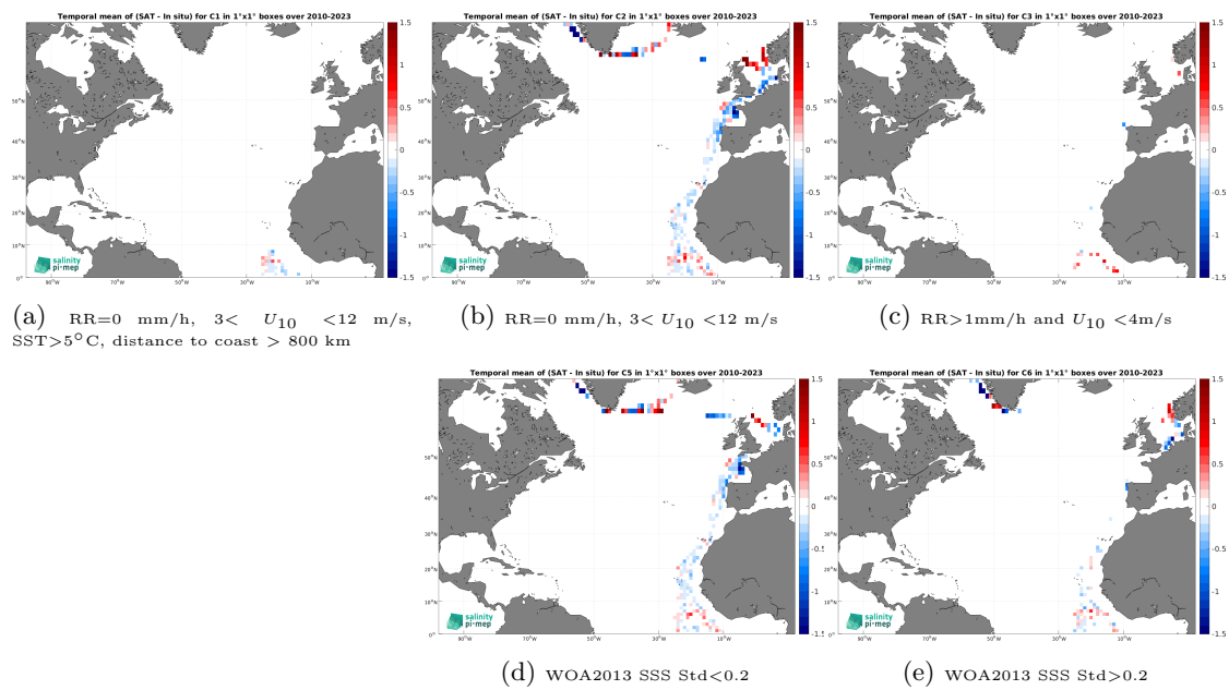
Figure 14: Temporal mean gridded over spatial boxes of size 1^\circ \times 1^\circ of \Delta\text{SSS} (SMOS SSS L3 v335 - Monthly - 25 km (CATDS-CPDC) - TSG (Polarstern)) for 5 different subdatasets corresponding to:RR=0 mm/h, 3 < U_{10} < 12 m/s, SST >5^\circ\text{C} , distance to coast > 800 km (a), RR=0 mm/h, 3 < U_{10} < 12 m/s (b), RR >1 mm/h and U_{10} < 4 m/s (c), WOA2013 SSS Std <0.2 (d), WOA2013 SSS Std >0.2 (e).
