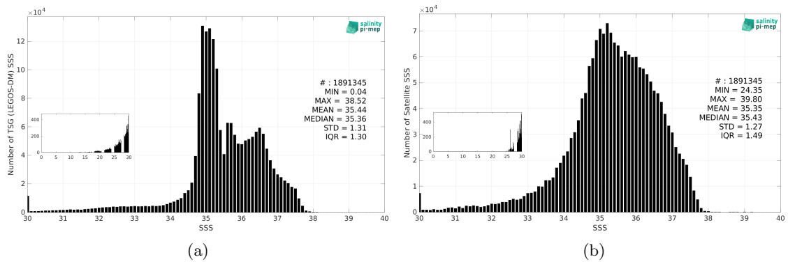
Figure 3: Histograms of SSS from TSG (LEGOS-DM) (a) and SMOS SSS L3 v335 - Monthly - 25 km (CATDS-CPDC) (b) considering all match-up pairs per bins of 0.1 over the North Atlantic Ocean Pi-MEP region and for the full satellite product period.
