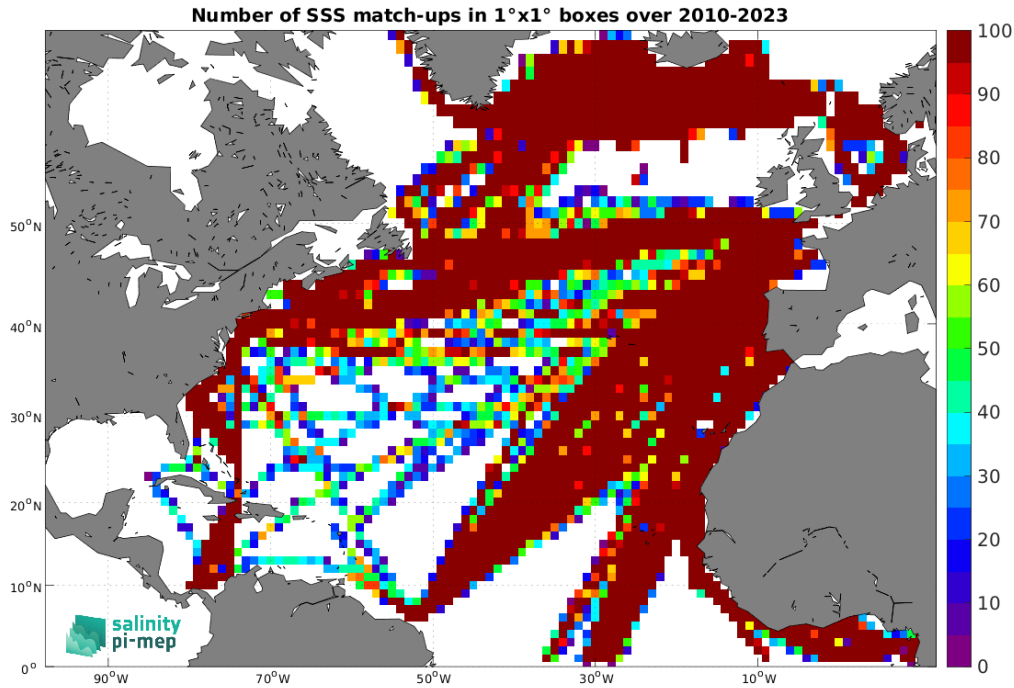
Figure 5: Number of SSS match-ups between TSG (LEGOS-DM) SSS and the SMOS SSS L3 v335 - Monthly - 25 km (CATDS-CPDC) SSS product for the North Atlantic Ocean Pi-MEP region over 1^\circ \times 1^\circ boxes and for the full satellite product period.
