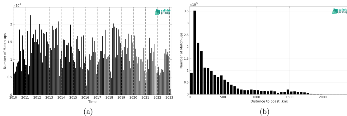
Figure 2: Number of match-ups between TSG (LEGOS-DM) and SMOS SSS L3 v335 - Monthly - 25 km (CATDS-CPDC) SSS as a function of time (a) and as function of the distance to coast (b) over the North Atlantic Ocean Pi-MEP region and for the full satellite product period.
