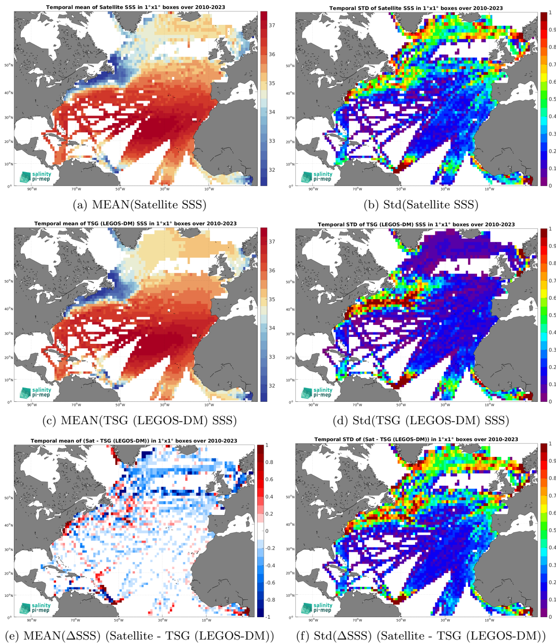
Figure 7: Temporal mean (left) and Std (right) of SSS from SMOS SSS L3 v335 - Monthly - 25 km (CATDS-CPDC) (top), TSG (LEGOS-DM) (middle), and of \Delta SSS (Satellite - TSG (LEGOS-DM)). Only match-up pairs are used to generate these maps.
