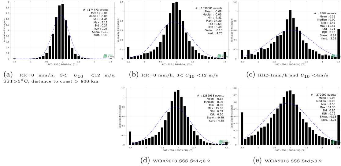
Figure 13: Normalized histogram of \Delta\text{SSS} (SMOS SSS L3 v335 - Monthly - 25 km (CATDS-CPDC) - TSG (LEGOS-DM)) for 5 different subdatasets corresponding to: RR=0 mm/h, 3 < U_{10} < 12 m/s, SST>5°C, distance to coast > 800 km (a), RR=0 mm/h, 3 < U_{10} < 12 m/s (b), RR>1mm/h and U_{10} < 4 m/s (c), WOA2013 SSS Std<0.2 (d), WOA2013 SSS Std>0.2 (e).
