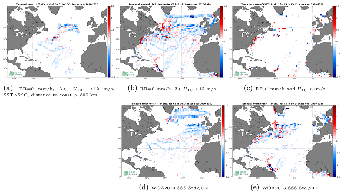
Figure 12: Temporal mean gridded over spatial boxes of size 1^\circ \times 1^\circ of \Delta SSS (SMOS SSS L3 v335 - Monthly - 25 km (CATDS-CPDC) - TSG (LEGOS-DM)) for 5 different subdatasets corresponding to: RR=0 mm/h, 3 < U_{10} < 12 m/s, SST > 5^\circ\text{C} , distance to coast > 800 km (a), RR=0 mm/h, 3 < U_{10} < 12 m/s (b), RR > 1 mm/h and U_{10} < 4 m/s (c), WOA2013 SSS Std < 0.2 (d), WOA2013 SSS Std > 0.2 (e).
