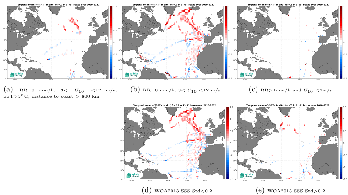
Figure 14: Temporal mean gridded over spatial boxes of size 1^\circ \times 1^\circ of \Delta\text{SSS} (SMOS SSS L3 v335 - Monthly - 25 km (CATDS-CPDC) - TSG (CSIC-UTM)) for 5 different subdatasets corresponding to:RR=0 mm/h, 3 < U_{10} < 12 m/s, SST >5^\circ\text{C} , distance to coast > 800 km (a), RR=0 mm/h, 3 < U_{10} < 12 m/s (b), RR >1 mm/h and U_{10} < 4 m/s (c), WOA2013 SSS Std <0.2 (d), WOA2013 SSS Std >0.2 (e).
