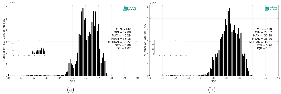
Figure 3: Histograms of SSS from TSG (CSIC-UTM) (a) and SMOS SSS L3 v335 - Monthly - 25 km (CATDS-CPDC) (b) considering all match-up pairs per bins of 0.1 over the North Atlantic Ocean Pi-MEP region and for the full satellite product period.
