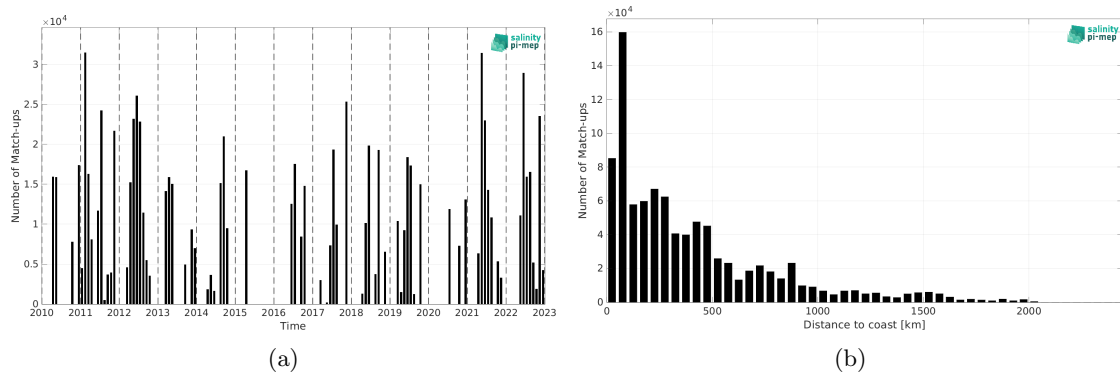
Figure 2: Number of match-ups between TSG (CSIC-UTM) and SMOS SSS L3 v335 - Monthly - 25 km (CATDS-CPDC) SSS as a function of time (a) and as function of the distance to coast (b) over the North Atlantic Ocean Pi-MEP region and for the full satellite product period.
