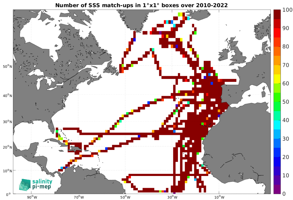
Figure 5: Number of SSS match-ups between TSG (CSIC-UTM) SSS and the SMOS SSS L3 v335 - Monthly - 25 km (CATDS-CPDC) SSS product for the North Atlantic Ocean Pi-MEP region over 1^\circ \times 1^\circ boxes and for the full satellite product period.
