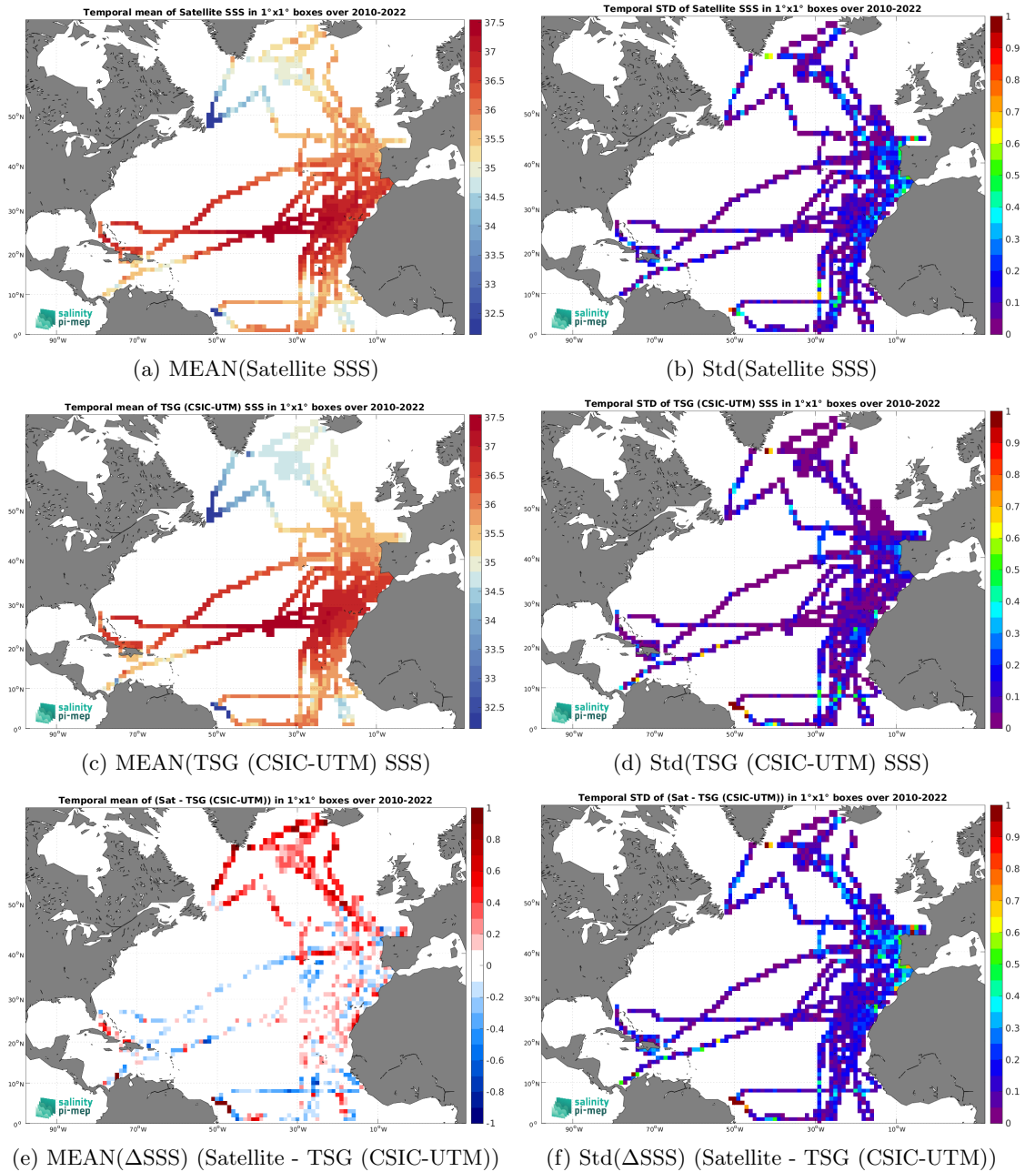
Figure 7: Temporal mean (left) and Std (right) of SSS from SMOS SSS L3 v335 - Monthly - 25 km (CATDS-CPDC) (top), TSG (CSIC-UTM) (middle), and of \Delta SSS (Satellite - TSG (CSIC-UTM)). Only match-up pairs are used to generate these maps.
