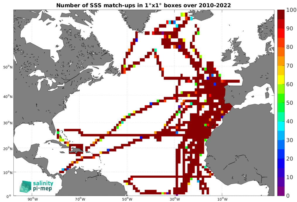
Figure 4: Number of SSS match-ups between TSG (CSIC-UTM) SSS and the SMOS SSS L3 v335 - Monthly - 25 km (CATDS-CPDC) SSS product for the North Atlantic Ocean Pi-MEP region over 1^\circ \times 1^\circ boxes and for the full satellite product period.
