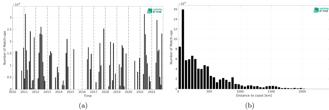
Figure 1: Number of match-ups between TSG (CSIC-UTM) and SMOS SSS L3 v335 - Monthly - 25 km (CATDS-CPDC) SSS as a function of time (a) and as function of the distance to coast (b) over the North Atlantic Ocean Pi-MEP region and for the full satellite product period.
