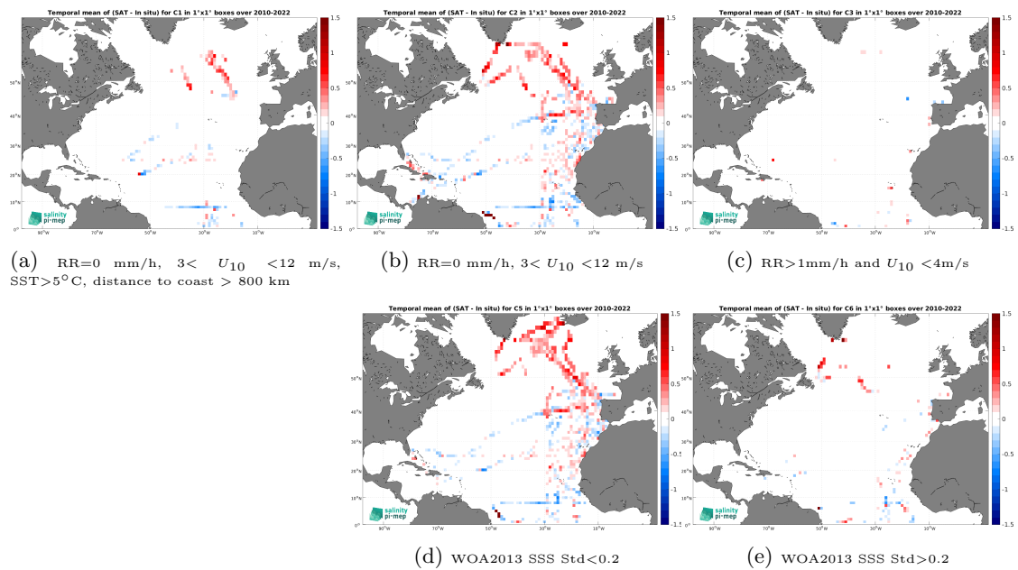
Figure 12: Temporal mean gridded over spatial boxes of size 1^\circ \times 1^\circ of \Delta\text{SSS} (SMOS SSS L3 v335 - Monthly - 25 km (CATDS-CPDC) - TSG (CSIC-UTM)) for 5 different subdatasets corresponding to:RR=0 mm/h, 3 < U_{10} < 12 m/s, SST >5^\circ\text{C} , distance to coast > 800 km (a), RR=0 mm/h, 3 < U_{10} < 12 m/s (b), RR >1 mm/h and U_{10} < 4 m/s (c), WOA2013 SSS Std <0.2 (d), WOA2013 SSS Std >0.2 (e).
