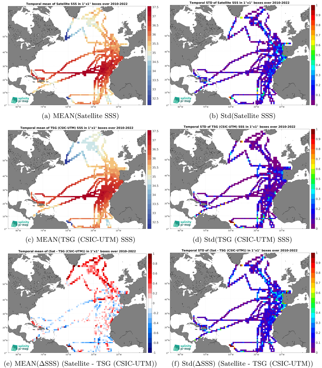
Figure 6: Temporal mean (left) and Std (right) of SSS from SMOS SSS L3 v335 - Monthly - 25 km (CATDS-CPDC) (top), TSG (CSIC-UTM) (middle), and of \Delta SSS (Satellite - TSG (CSIC-UTM)). Only match-up pairs are used to generate these maps.
