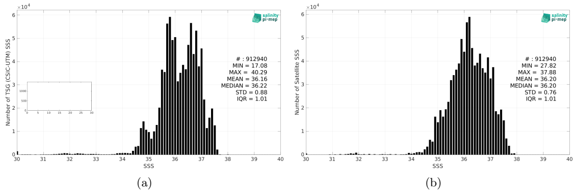
Figure 2: Histograms of SSS from TSG (CSIC-UTM) (a) and SMOS SSS L3 v335 - Monthly - 25 km (CATDS-CPDC) (b) considering all match-up pairs per bins of 0.1 over the North Atlantic Ocean Pi-MEP region and for the full satellite product period.
