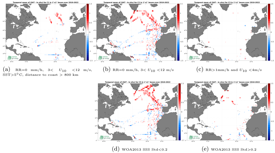
Figure 12: Temporal mean gridded over spatial boxes of size 1^\circ \times 1^\circ of \Delta SSS (SMOS SSS L3 v335 - Monthly - 25 km (CATDS-CPDC) - TSG (CSIC-UTM)) for 5 different subdatasets corresponding to:RR=0 mm/h, 3 < U_{10} < 12 m/s, SST >5^\circ\text{C} , distance to coast > 800 km (a), RR=0 mm/h, 3 < U_{10} < 12 m/s (b), RR >1 mm/h and U_{10} < 4 m/s (c), WOA2013 SSS Std <0.2 (d), WOA2013 SSS Std >0.2 (e).
