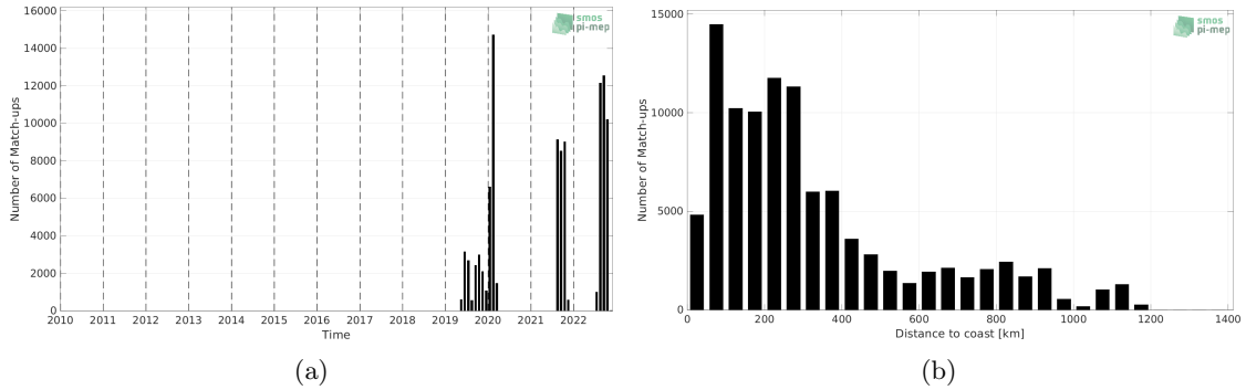
Figure 1: Number of match-ups between Saildrone and SMOS SSS L3 v335 - Monthly - 25 km (CATDS-CPDC) SSS as a function of time (a) and as function of the distance to coast (b) over the North Atlantic Ocean Pi-MEP region and for the full satellite product period.
