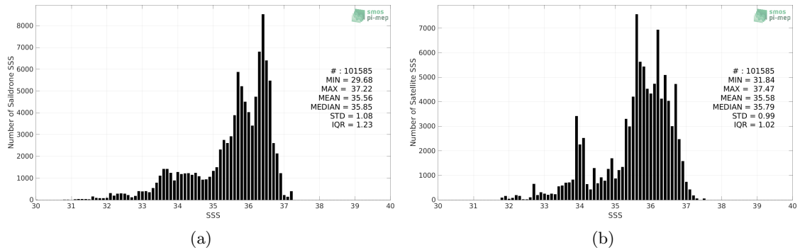
Figure 2: Histograms of SSS from Saildrone (a) and SMOS SSS L3 v335 - Monthly - 25 km (CATDS-CPDC) (b) considering all match-up pairs per bins of 0.1 over the North Atlantic Ocean Pi-MEP region and for the full satellite product period.
