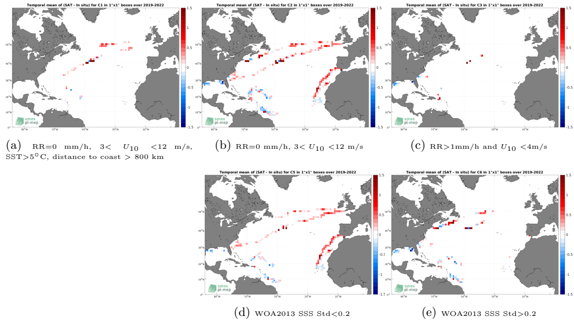
Figure 12: Temporal mean gridded over spatial boxes of size 1^\circ \times 1^\circ of \Delta\text{SSS} (SMOS SSS L3 v335 - Monthly - 25 km (CATDS-CPDC) - Saildrone) for 5 different subdatasets corresponding to:RR=0 mm/h, 3 < U_{10} < 12 m/s, SST >5^\circ\text{C} , distance to coast > 800 km (a), RR=0 mm/h, 3 < U_{10} < 12 m/s (b), RR >1 mm/h and U_{10} < 4 m/s (c), WOA2013 SSS Std <0.2 (d), WOA2013 SSS Std >0.2 (e).
