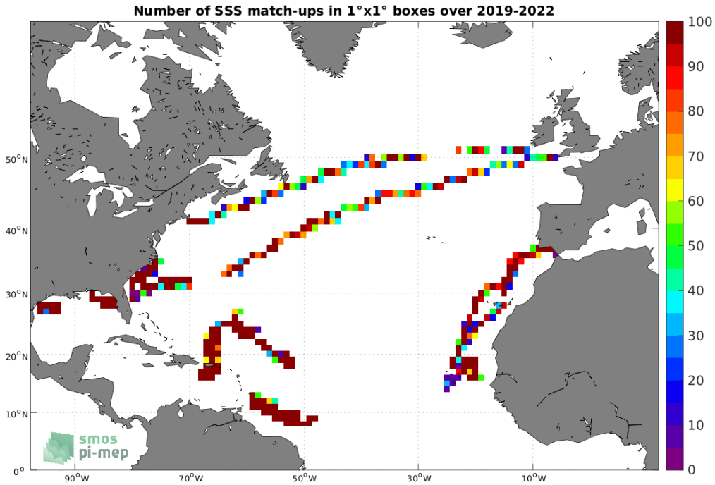
Figure 4: Number of SSS match-ups between Saildrone SSS and the SMOS SSS L3 v335 - Monthly - 25 km (CATDS-CPDC) SSS product for the North Atlantic Ocean Pi-MEP region over 1^\circ \times 1^\circ boxes and for the full satellite product period.
