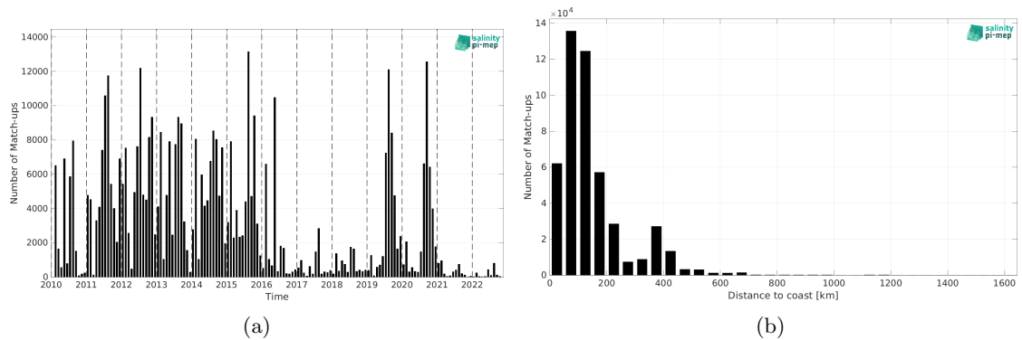
Figure 2: Number of match-ups between ICES and SMOS SSS L3 v335 - Monthly - 25 km (CATDS-CPDC) SSS as a function of time (a) and as function of the distance to coast (b) over the North Atlantic Ocean Pi-MEP region and for the full satellite product period.
