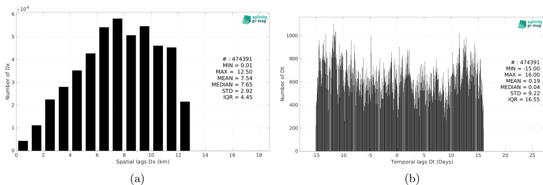
Figure 6: Histograms of the spatial (a) and temporal (b) lags between the location/time of the ICES measurement and the date of the corresponding SMOS SSS L3 v335 - Monthly - 25 km (CATDS-CPDC) SSS pixel.
