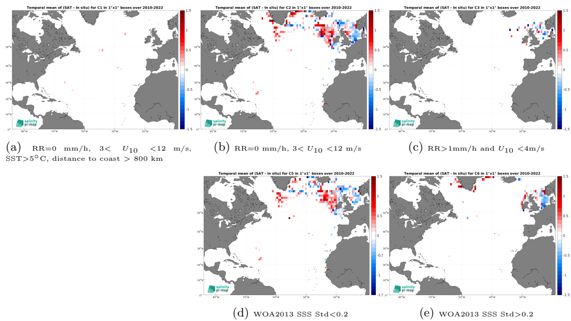
Figure 14: Temporal mean gridded over spatial boxes of size 1^\circ \times 1^\circ of \Delta\text{SSS} (SMOS SSS L3 v335 - Monthly - 25 km (CATDS-CPDC) - ICES) for 5 different subdatasets corresponding to:RR=0 mm/h, 3 < U_{10} < 12 m/s, SST >5^\circ\text{C} , distance to coast > 800 km (a), RR=0 mm/h, 3 < U_{10} < 12 m/s (b), RR >1 mm/h and U_{10} < 4 m/s (c), WOA2013 SSS Std <0.2 (d), WOA2013 SSS Std >0.2 (e).
