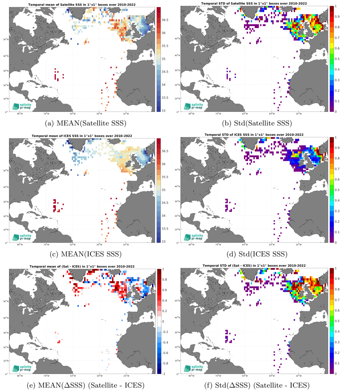
Figure 7: Temporal mean (left) and Std (right) of SSS from SMOS SSS L3 v335 - Monthly - 25 km (CATDS-CPDC) (top), ICES (middle), and of \Delta SSS (Satellite - ICES). Only match-up pairs are used to generate these maps.
