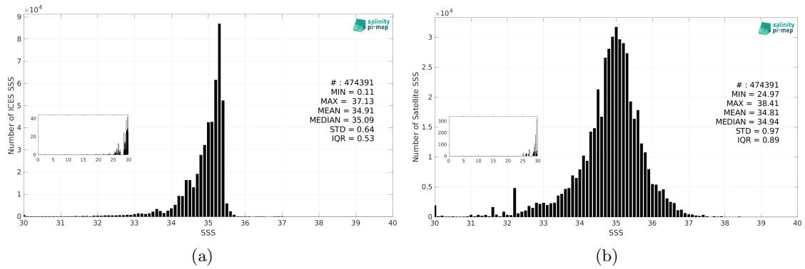
Figure 3: Histograms of SSS from ICES (a) and SMOS SSS L3 v335 - Monthly - 25 km (CATDS-CPDC) (b) considering all match-up pairs per bins of 0.1 over the North Atlantic Ocean Pi-MEP region and for the full satellite product period.
