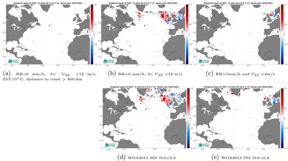
Figure 12: Temporal mean gridded over spatial boxes of size 1^\circ \times 1^\circ of \Delta SSS (SMOS SSS L3 v335 - Monthly - 25 km (CATDS-CPDC) - ICES) for 5 different subdatasets corresponding to:RR=0 mm/h, 3 < U_{10} < 12 m/s, SST >5^\circ C, distance to coast > 800 km (a), RR=0 mm/h, 3 < U_{10} < 12 m/s (b), RR >1 mm/h and U_{10} < 4 m/s (c), WOA2013 SSS Std <0.2 (d), WOA2013 SSS Std >0.2 (e).
