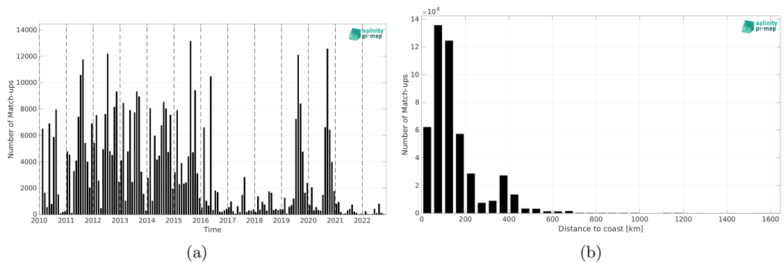
Figure 1: Number of match-ups between ICES and SMOS SSS L3 v335 - Monthly - 25 km (CATDS-CPDC) SSS as a function of time (a) and as function of the distance to coast (b) over the North Atlantic Ocean Pi-MEP region and for the full satellite product period.
