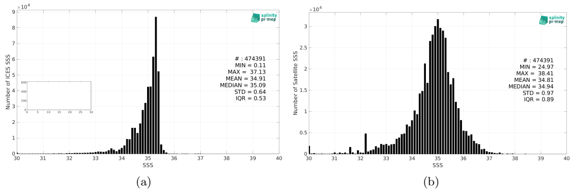
Figure 2: Histograms of SSS from ICES (a) and SMOS SSS L3 v335 - Monthly - 25 km (CATDS-CPDC) (b) considering all match-up pairs per bins of 0.1 over the North Atlantic Ocean Pi-MEP region and for the full satellite product period.
