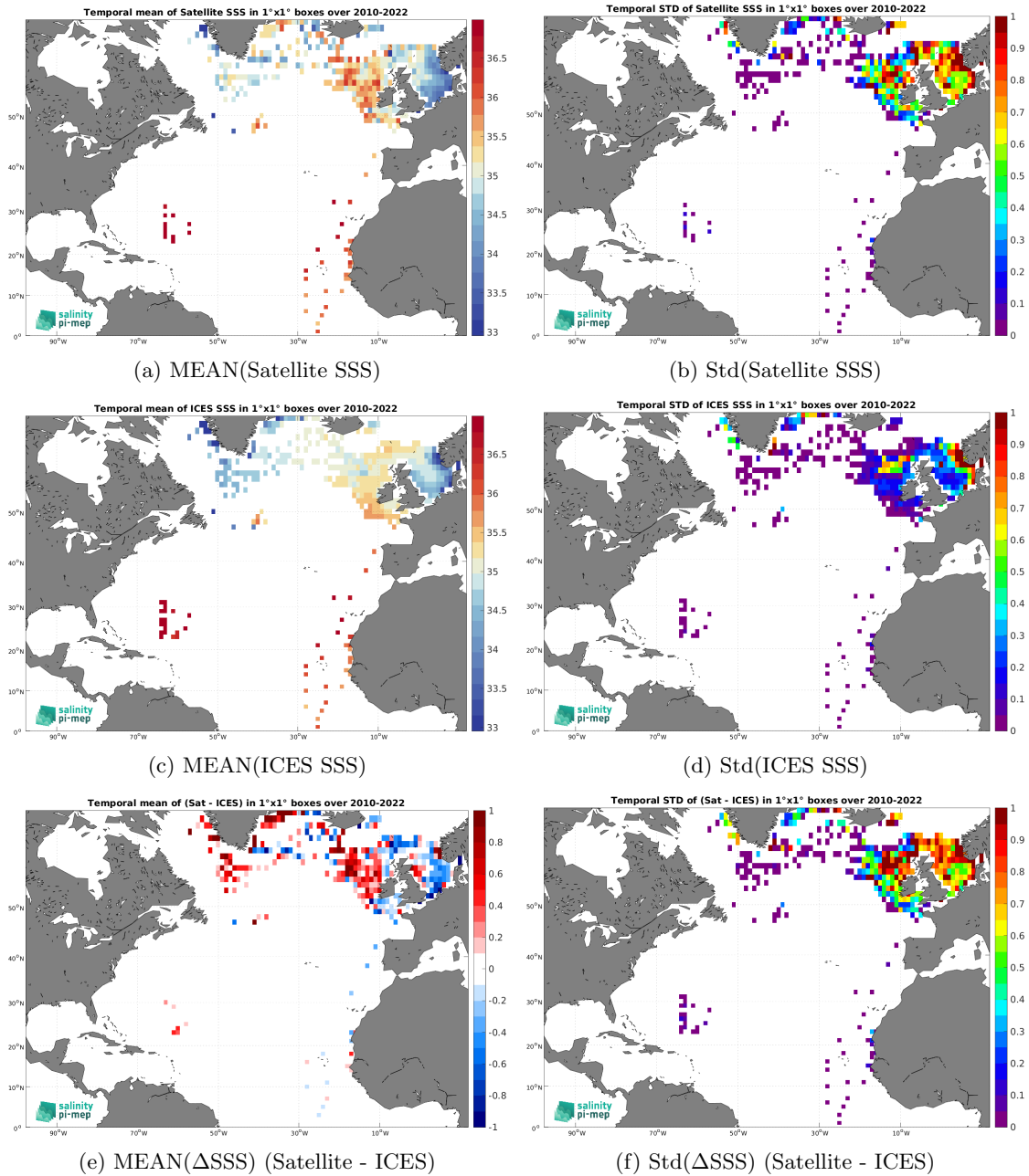
Figure 6: Temporal mean (left) and Std (right) of SSS from SMOS SSS L3 v335 - Monthly - 25 km (CATDS-CPDC) (top), ICES (middle), and of \Delta SSS (Satellite - ICES). Only match-up pairs are used to generate these maps.
