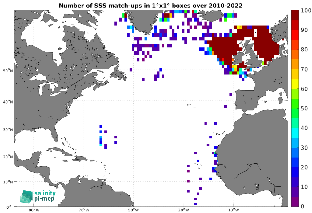
Figure 4: Number of SSS match-ups between ICES SSS and the SMOS SSS L3 v335 - Monthly - 25 km (CATDS-CPDC) SSS product for the North Atlantic Ocean Pi-MEP region over 1^\circ \times 1^\circ boxes and for the full satellite product period.
