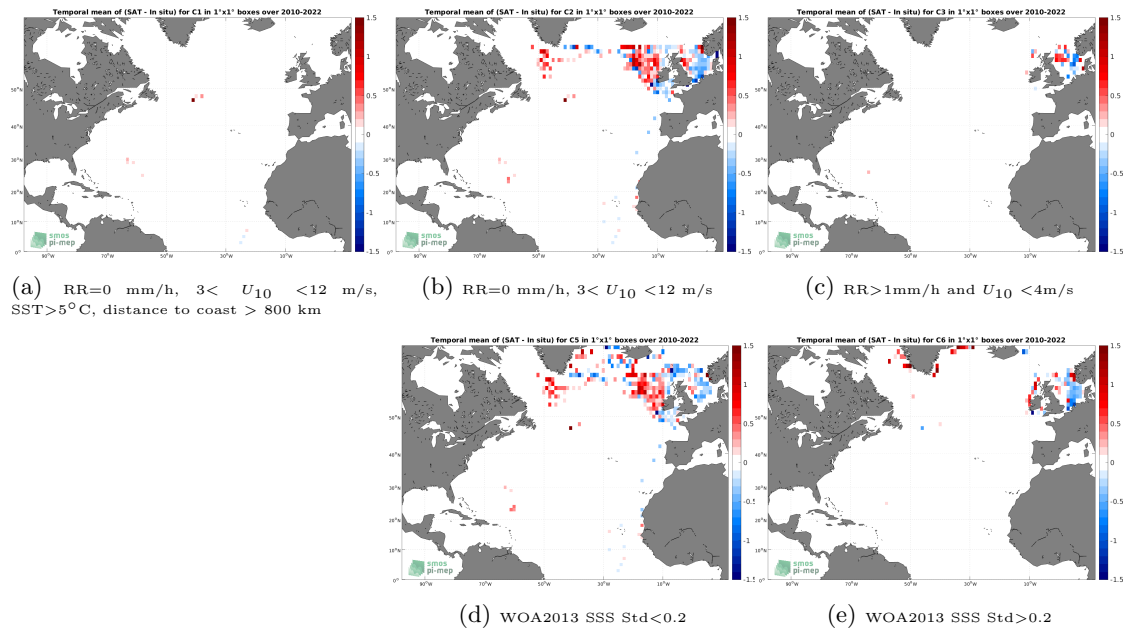
Figure 12: Temporal mean gridded over spatial boxes of size 1^\circ \times 1^\circ of \Delta\text{SSS} (SMOS SSS L3 v335 - Monthly - 25 km (CATDS-CPDC) - ICES) for 5 different subdatasets corresponding to:RR=0 mm/h, 3 < U_{10} < 12 m/s, SST >5^\circ\text{C} , distance to coast > 800 km (a), RR=0 mm/h, 3 < U_{10} < 12 m/s (b), RR >1 mm/h and U_{10} < 4 m/s (c), WOA2013 SSS Std <0.2 (d), WOA2013 SSS Std >0.2 (e).
