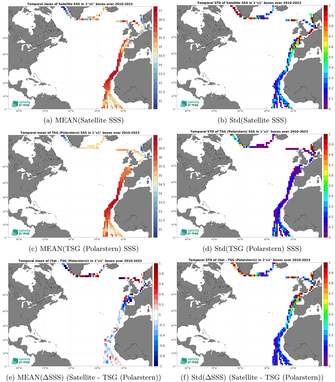
Figure 7: Temporal mean (left) and Std (right) of SSS from SMOS SSS L3 v335 - 10 Days - 25 km (CATDS-CPDC) (top), TSG (Polarstern) (middle), and of \Delta SSS (Satellite - TSG (Polarstern)). Only match-up pairs are used to generate these maps.
