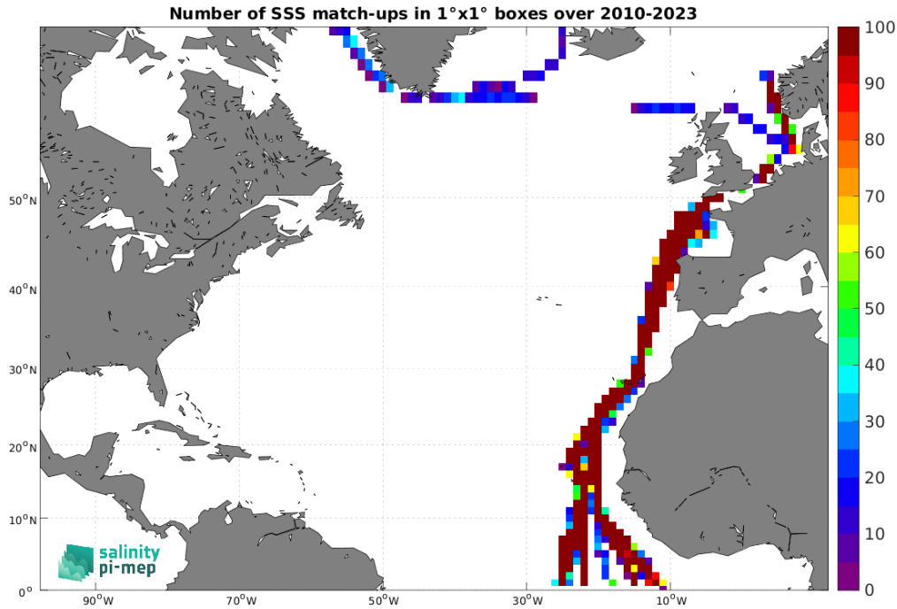
Figure 5: Number of SSS match-ups between TSG (Polarstern) SSS and the SMOS SSS L3 v335 - 10 Days - 25 km (CATDS-CPDC) SSS product for the North Atlantic Ocean Pi-MEP region over 1^\circ \times 1^\circ boxes and for the full satellite product period.
