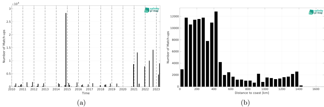
Figure 2: Number of match-ups between TSG (Polarstern) and SMOS SSS L3 v335 - 10 Days - 25 km (CATDS-CPDC) SSS as a function of time (a) and as function of the distance to coast (b) over the North Atlantic Ocean Pi-MEP region and for the full satellite product period.
