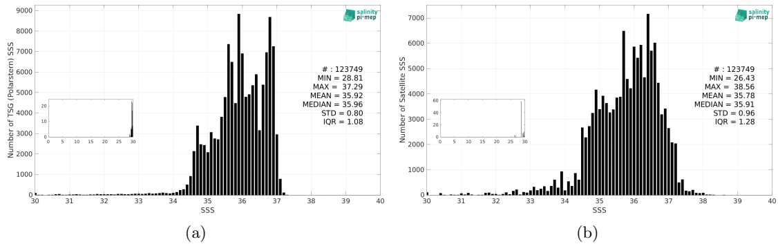
Figure 3: Histograms of SSS from TSG (Polarstern) (a) and SMOS SSS L3 v335 - 10 Days - 25 km (CATDS-CPDC) (b) considering all match-up pairs per bins of 0.1 over the North Atlantic Ocean Pi-MEP region and for the full satellite product period.
