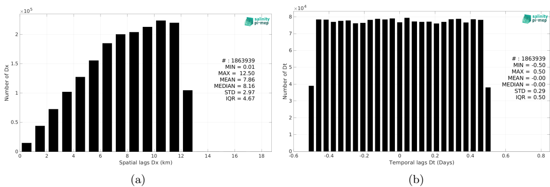
Figure 6: Histograms of the spatial (a) and temporal (b) lags between the location/time of the TSG (LEGOS-DM) measurement and the date of the corresponding SMOS SSS L3 v335 - 10 Days - 25 km (CATDS-CPDC) SSS pixel.
