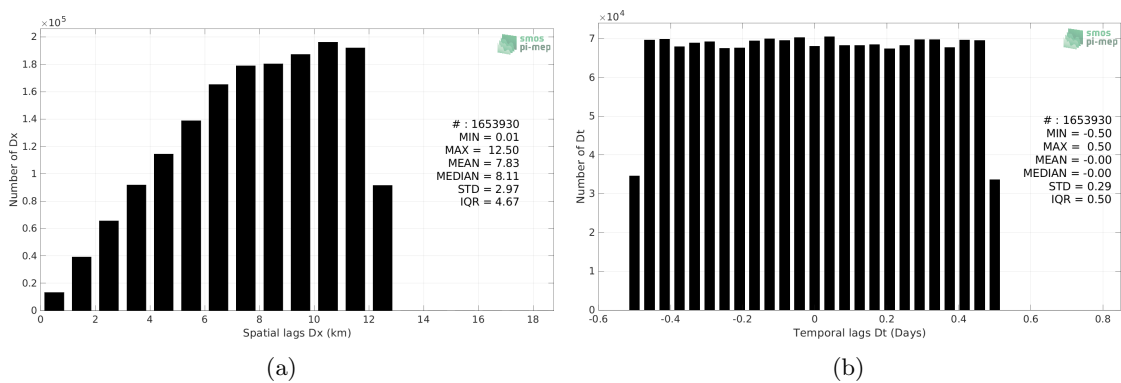
Figure 5: Histograms of the spatial (a) and temporal (b) lags between the location/time of the TSG (LEGOS-DM) measurement and the date of the corresponding SMOS SSS L3 v335 - 10 Days - 25 km (CATDS-CPDC) SSS pixel.
