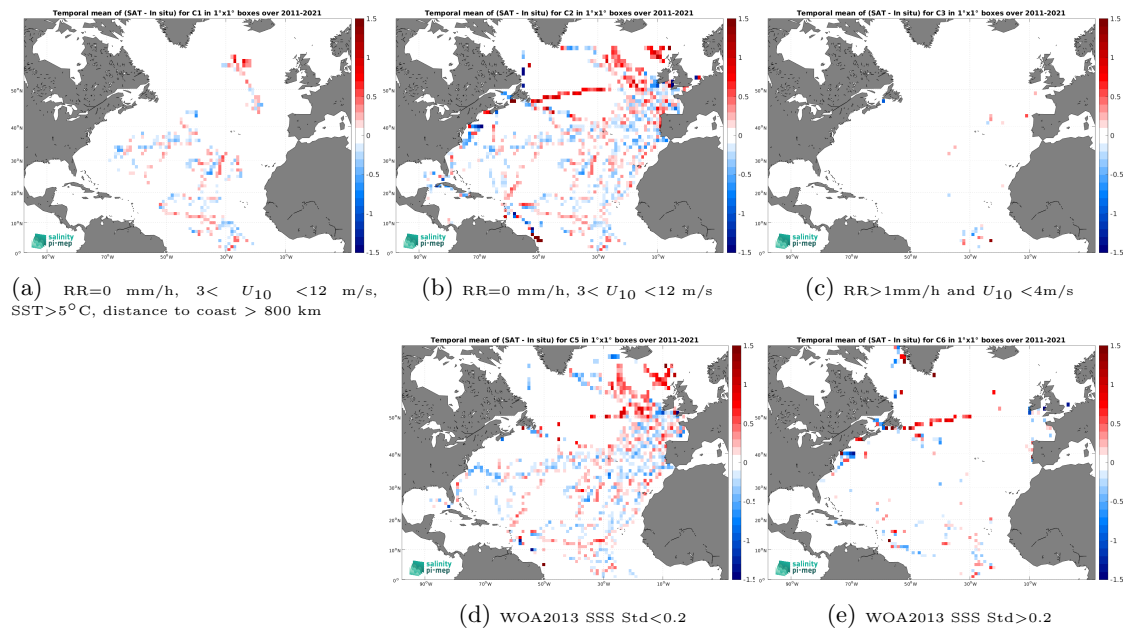
Figure 12: Temporal mean gridded over spatial boxes of size 1^\circ \times 1^\circ of \Delta\text{SSS} (SMOS SSS L3 v335 - 10 Days - 25 km (CATDS-CPDC) - TSG (GOSUD-Sailing-ship)) for 5 different subdatasets corresponding to:RR=0 mm/h, 3 < U_{10} < 12 m/s, SST >5^\circ\text{C} , distance to coast > 800 km (a), RR=0 mm/h, 3 < U_{10} < 12 m/s (b), RR >1 mm/h and U_{10} < 4 m/s (c), WOA2013 SSS Std <0.2 (d), WOA2013 SSS Std >0.2 (e).
