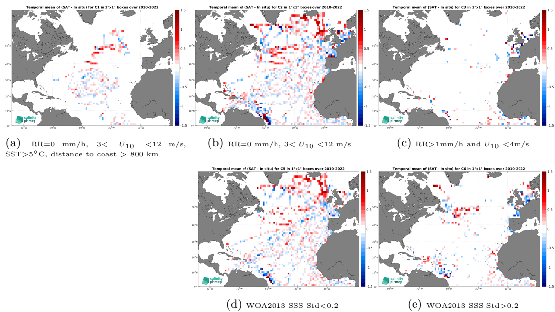
Figure 14: Temporal mean gridded over spatial boxes of size 1^\circ \times 1^\circ of \Delta SSS (SMOS SSS L3 v335 - 10 Days - 25 km (CATDS-CPDC) - TSG (GOSUD-Research-vessel)) for 5 different subdatasets corresponding to:RR=0 mm/h, 3 < U_{10} < 12 m/s, SST >5^\circ\text{C} , distance to coast > 800 km (a), RR=0 mm/h, 3 < U_{10} < 12 m/s (b), RR >1 mm/h and U_{10} < 4 m/s (c), WOA2013 SSS Std <0.2 (d), WOA2013 SSS Std >0.2 (e).
