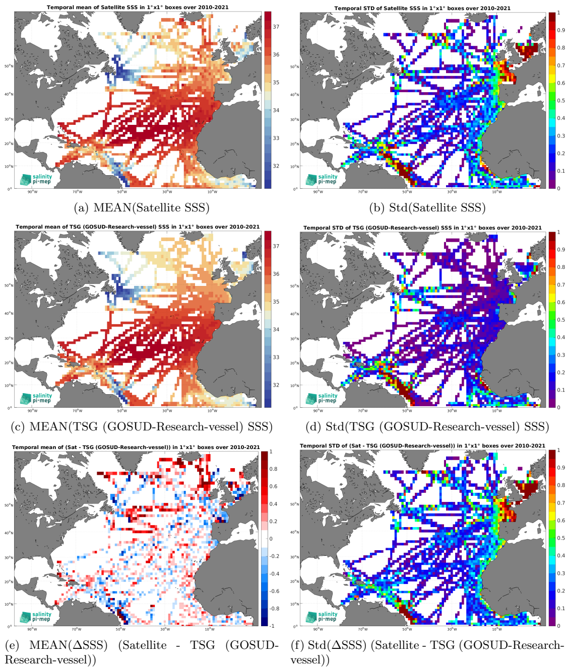
Figure 7: Temporal mean (left) and Std (right) of SSS from SMOS SSS L3 v335 - 10 Days - 25 km (CATDS-CPDC) (top), TSG (GOSUD-Research-vessel) (middle), and of \Delta SSS (Satellite - TSG (GOSUD-Research-vessel)). Only match-up pairs are used to generate these maps.
