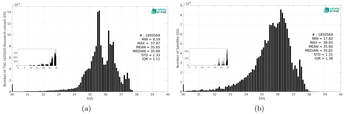
Figure 3: Histograms of SSS from TSG (GOSUD-Research-vessel) (a) and SMOS SSS L3 v335 - 10 Days - 25 km (CATDS-CPDC) (b) considering all match-up pairs per bins of 0.1 over the North Atlantic Ocean Pi-MEP region and for the full satellite product period.
