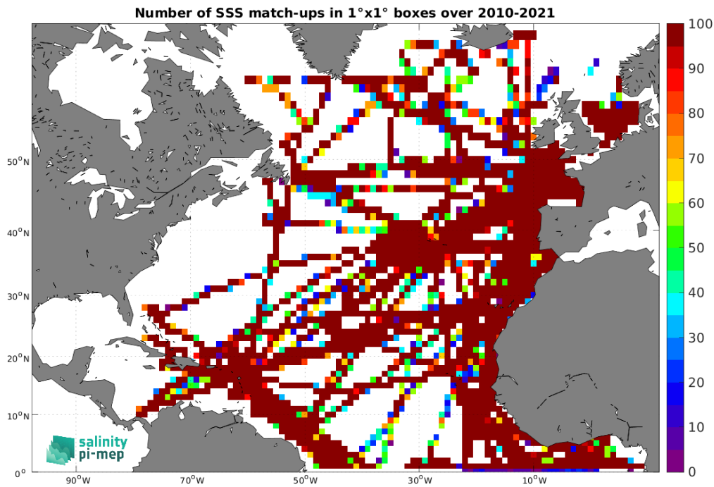
Figure 5: Number of SSS match-ups between TSG (GOSUD-Research-vessel) SSS and the SMOS SSS L3 v335 - 10 Days - 25 km (CATDS-CPDC) SSS product for the North Atlantic Ocean Pi-MEP region over 1^\circ \times 1^\circ boxes and for the full satellite product period.
