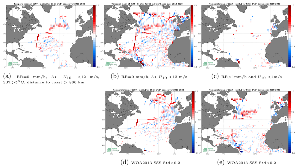
Figure 12: Temporal mean gridded over spatial boxes of size 1^\circ \times 1^\circ of \Delta\text{SSS} (SMOS SSS L3 v335 - 10 Days - 25 km (CATDS-CPDC) - TSG (GOSUD-Research-vessel)) for 5 different subdatasets corresponding to: RR=0 mm/h, 3 < U_{10} < 12 m/s, SST > 5°C, distance to coast > 800 km (a), RR=0 mm/h, 3 < U_{10} < 12 m/s (b), RR > 1mm/h and U_{10} < 4 m/s (c), WOA2013 SSS Std < 0.2 (d), WOA2013 SSS Std > 0.2 (e).
