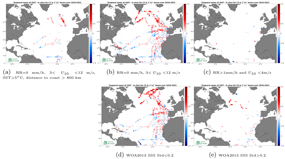
Figure 12: Temporal mean gridded over spatial boxes of size 1^\circ \times 1^\circ of \Delta SSS (SMOS SSS L3 v335 - 10 Days - 25 km (CATDS-CPDC) - TSG (CSIC-UTM)) for 5 different subdatasets corresponding to:RR=0 mm/h, 3 < U_{10} < 12 m/s, SST >5^\circ C, distance to coast > 800 km (a), RR=0 mm/h, 3 < U_{10} < 12 m/s (b), RR >1 mm/h and U_{10} < 4 m/s (c), WOA2013 SSS Std <0.2 (d), WOA2013 SSS Std >0.2 (e).
