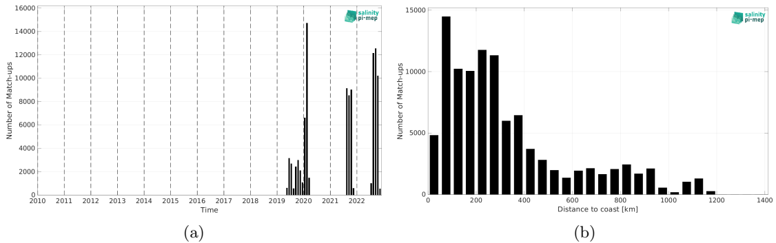
Figure 2: Number of match-ups between Saildrone and SMOS SSS L3 v335 - 10 Days - 25 km (CATDS-CPDC) SSS as a function of time (a) and as function of the distance to coast (b) over the North Atlantic Ocean Pi-MEP region and for the full satellite product period.
