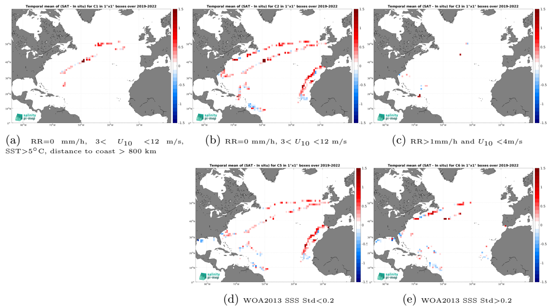
Figure 14: Temporal mean gridded over spatial boxes of size 1^\circ \times 1^\circ of \Delta\text{SSS} (SMOS SSS L3 v335 - 10 Days - 25 km (CATDS-CPDC) - Saildrone) for 5 different subdatasets corresponding to:RR=0 mm/h, 3 < U_{10} < 12 m/s, SST > 5°C, distance to coast > 800 km (a), RR=0 mm/h, 3 < U_{10} < 12 m/s (b), RR > 1mm/h and U_{10} < 4 m/s (c), WOA2013 SSS Std < 0.2 (d), WOA2013 SSS Std > 0.2 (e).
