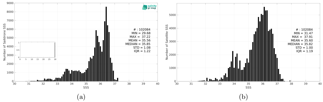
Figure 3: Histograms of SSS from Saildrone (a) and SMOS SSS L3 v335 - 10 Days - 25 km (CATDS-CPDC) (b) considering all match-up pairs per bins of 0.1 over the North Atlantic Ocean Pi-MEP region and for the full satellite product period.
