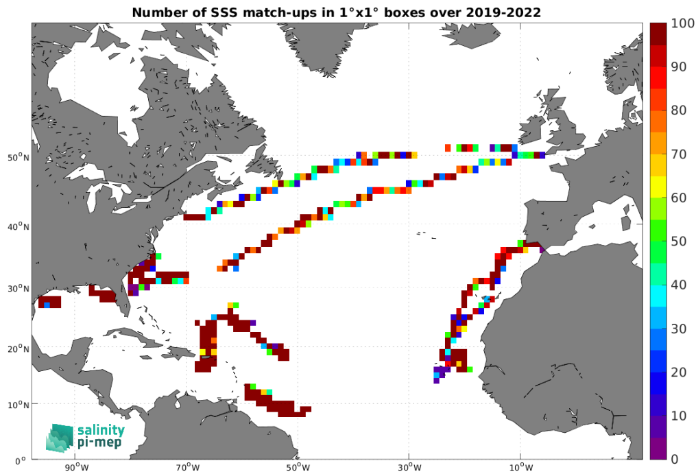
Figure 5: Number of SSS match-ups between Saildrone SSS and the SMOS SSS L3 v335 - 10 Days - 25 km (CATDS-CPDC) SSS product for the North Atlantic Ocean Pi-MEP region over 1^\circ \times 1^\circ boxes and for the full satellite product period.
