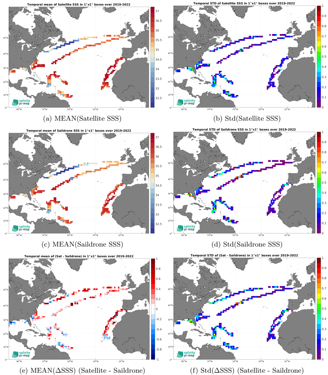
Figure 7: Temporal mean (left) and Std (right) of SSS from SMOS SSS L3 v335 - 10 Days - 25 km (CATDS-CPDC) (top), Saildrone (middle), and of \Delta SSS (Satellite - Saildrone). Only match-up pairs are used to generate these maps.
