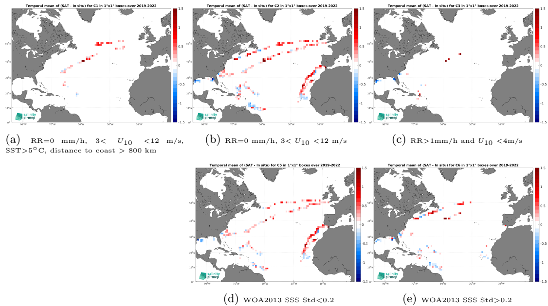
Figure 12: Temporal mean gridded over spatial boxes of size 1^\circ \times 1^\circ of \Delta\text{SSS} (SMOS SSS L3 v335 - 10 Days - 25 km (CATDS-CPDC) - Saildrone) for 5 different subdatasets corresponding to:RR=0 mm/h, 3 < U_{10} < 12 m/s, SST >5^\circ\text{C} , distance to coast > 800 km (a), RR=0 mm/h, 3 < U_{10} < 12 m/s (b), RR >1 mm/h and U_{10} < 4 m/s (c), WOA2013 SSS Std <0.2 (d), WOA2013 SSS Std >0.2 (e).
