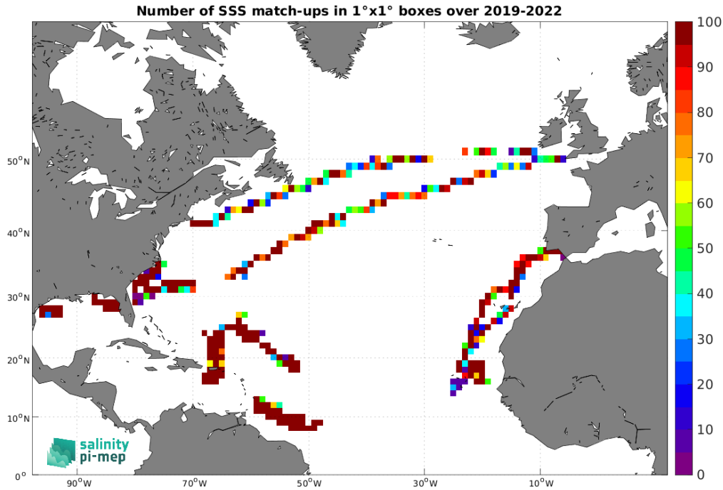
Figure 4: Number of SSS match-ups between Saildrone SSS and the SMOS SSS L3 v335 - 10 Days - 25 km (CATDS-CPDC) SSS product for the North Atlantic Ocean Pi-MEP region over 1^\circ \times 1^\circ boxes and for the full satellite product period.
