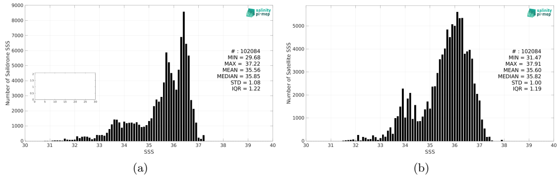
Figure 2: Histograms of SSS from Saildrone (a) and SMOS SSS L3 v335 - 10 Days - 25 km (CATDS-CPDC) (b) considering all match-up pairs per bins of 0.1 over the North Atlantic Ocean Pi-MEP region and for the full satellite product period.
