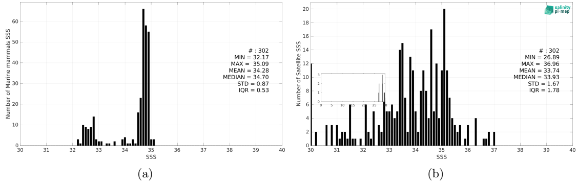
Figure 3: Histograms of SSS from Marine mammals (a) and SMOS SSS L3 v335 - 10 Days - 25 km (CATDS-CPDC) (b) considering all match-up pairs per bins of 0.1 over the North Atlantic Ocean Pi-MEP region and for the full satellite product period.
