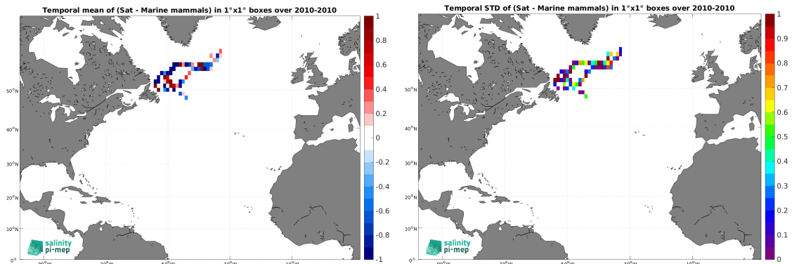
(e) MEAN( \Delta SSS) (Satellite - Marine mammals)
