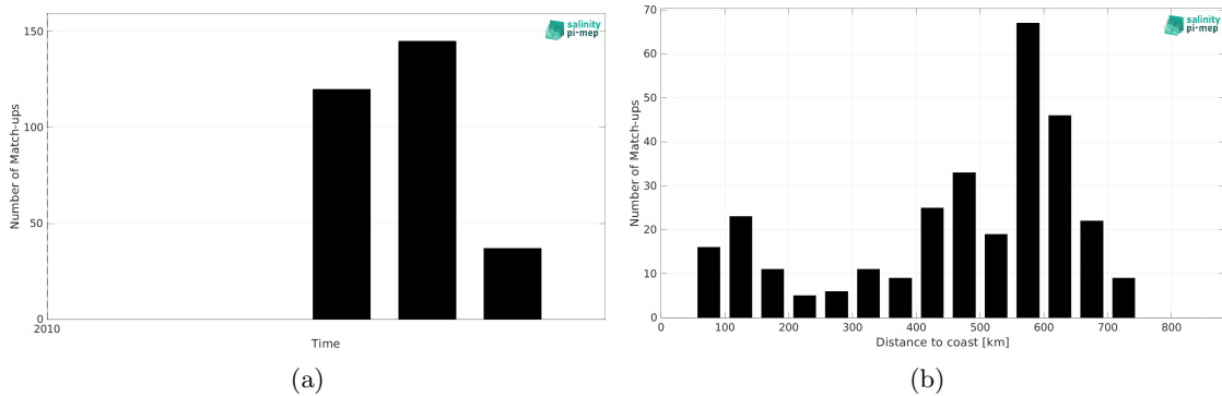
Figure 2: Number of match-ups between Marine mammals and SMOS SSS L3 v335 - 10 Days - 25 km (CATDS-CPDC) SSS as a function of time (a) and as function of the distance to coast (b) over the North Atlantic Ocean Pi-MEP region and for the full satellite product period.
