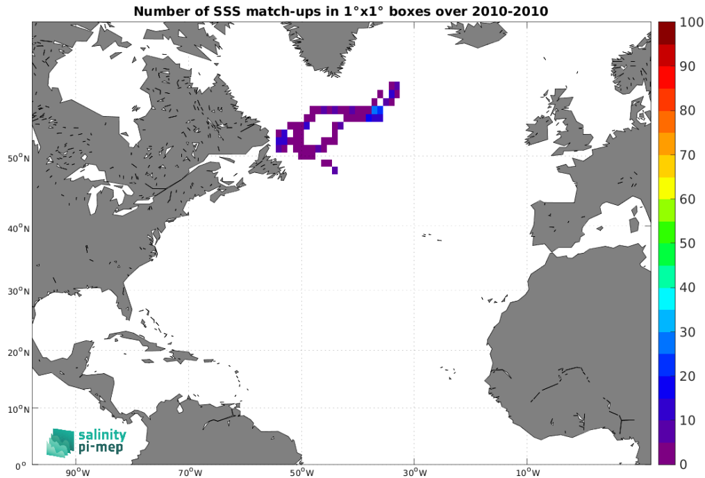
Figure 5: Number of SSS match-ups between Marine mammals SSS and the SMOS SSS L3 v335 - 10 Days - 25 km (CATDS-CPDC) SSS product for the North Atlantic Ocean Pi-MEP region over 1^\circ \times 1^\circ boxes and for the full satellite product period.
