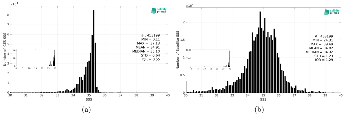
Figure 3: Histograms of SSS from ICES (a) and SMOS SSS L3 v335 - 10 Days - 25 km (CATDS-CPDC) (b) considering all match-up pairs per bins of 0.1 over the North Atlantic Ocean Pi-MEP region and for the full satellite product period.
