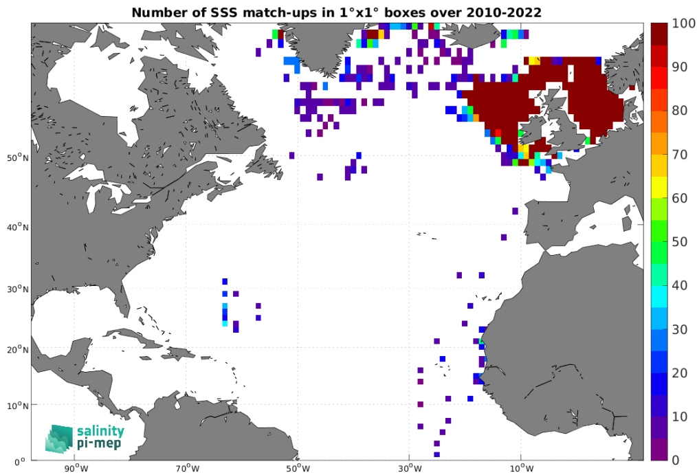
Figure 5: Number of SSS match-ups between ICES SSS and the SMOS SSS L3 v335 - 10 Days - 25 km (CATDS-CPDC) SSS product for the North Atlantic Ocean Pi-MEP region over 1^\circ \times 1^\circ boxes and for the full satellite product period.
