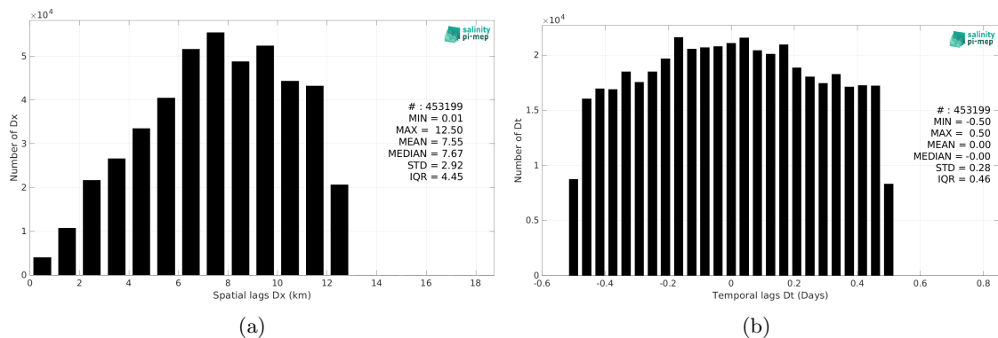
Figure 6: Histograms of the spatial (a) and temporal (b) lags between the location/time of the ICES measurement and the date of the corresponding SMOS SSS L3 v335 - 10 Days - 25 km (CATDS-CPDC) SSS pixel.
