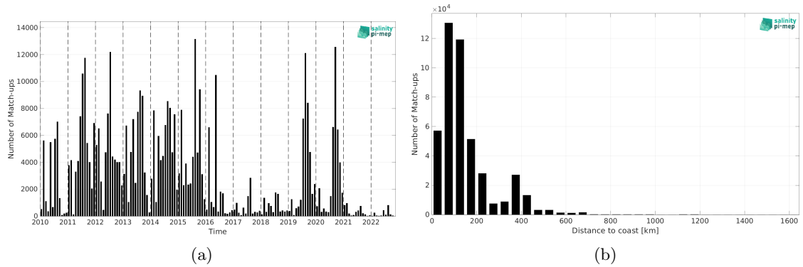
Figure 2: Number of match-ups between ICES and SMOS SSS L3 v335 - 10 Days - 25 km (CATDS-CPDC) SSS as a function of time (a) and as function of the distance to coast (b) over the North Atlantic Ocean Pi-MEP region and for the full satellite product period.
