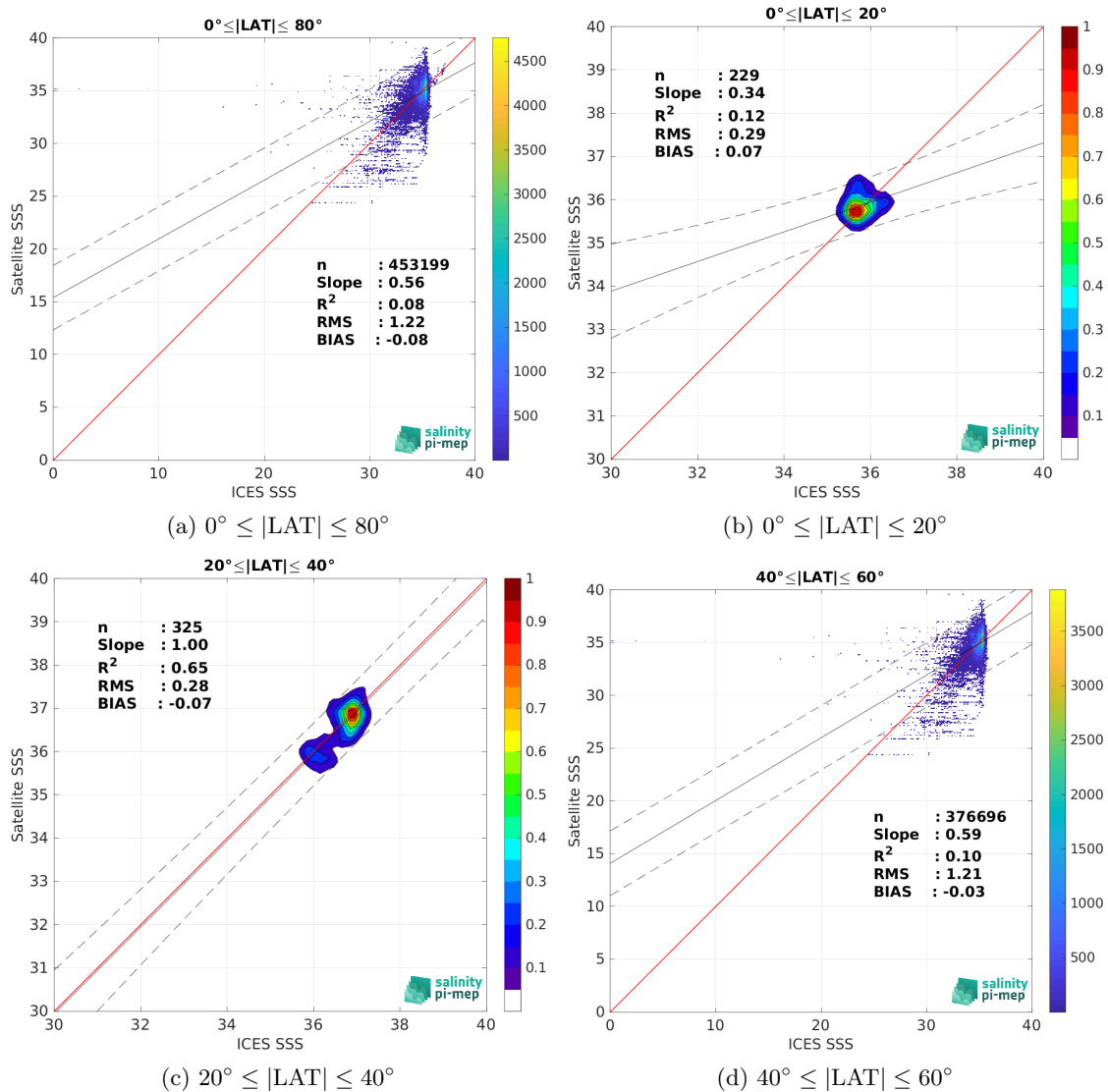
Figure 10: Contour maps of the concentration of SMOS SSS L3 v335 - 10 Days - 25 km (CATDS-CPDC) SSS (y-axis) versus ICES SSS (x-axis) at match-up pairs for different latitude bands. For each plot, the red line shows x=y . The black thin and dashed lines indicate a linear fit through the data cloud and the \pm 95\% confidence levels, respectively. The number match-up pairs n , the slope and R^2 coefficient of the linear fit, the root mean square (RMS) and the mean bias between satellite and in situ data are indicated for each latitude band in each plots.
