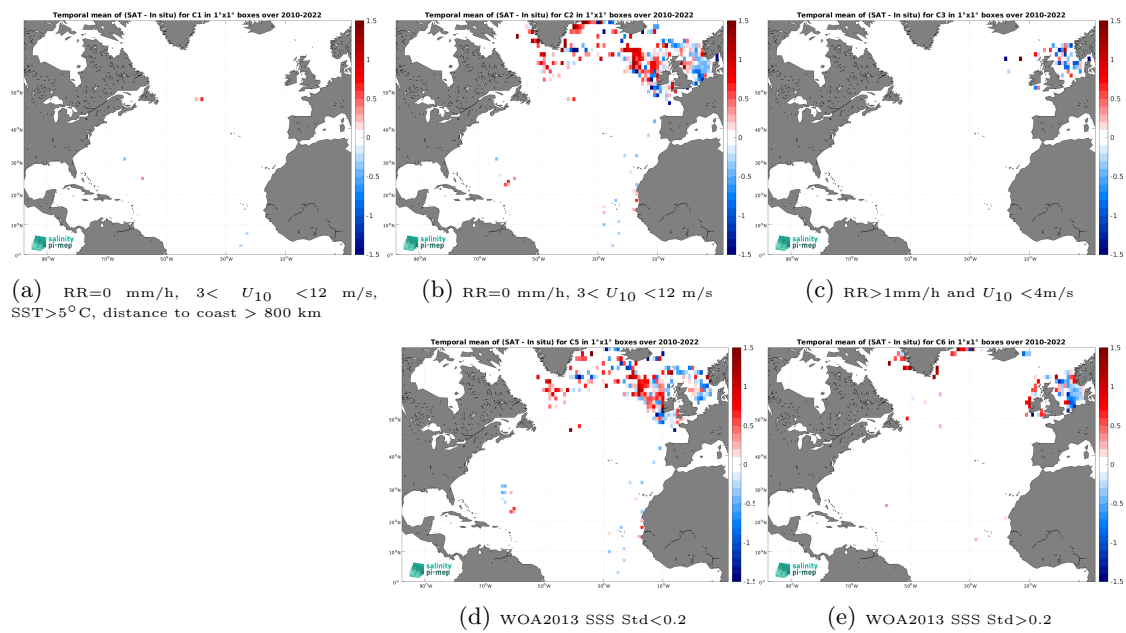
Figure 14: Temporal mean gridded over spatial boxes of size 1^\circ \times 1^\circ of \Delta\text{SSS} (SMOS SSS L3 v335 - 10 Days - 25 km (CATDS-CPDC) - ICES) for 5 different subdatasets corresponding to:RR=0 mm/h, 3 < U_{10} < 12 m/s, SST >5^\circ\text{C} , distance to coast > 800 km (a), RR=0 mm/h, 3 < U_{10} < 12 m/s (b), RR >1 mm/h and U_{10} < 4 m/s (c), WOA2013 SSS Std <0.2 (d), WOA2013 SSS Std >0.2 (e).
