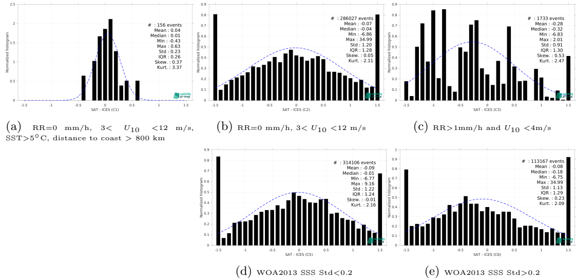
Figure 15: Normalized histogram of \Delta SSS (SMOS SSS L3 v335 - 10 Days - 25 km (CATDS-CPDC) - ICES) for 5 different subdatasets corresponding to: RR=0 mm/h, 3 < U_{10} < 12 m/s, SST>5°C, distance to coast > 800 km (a), RR=0 mm/h, 3 < U_{10} < 12 m/s (b), RR>1mm/h and U_{10} < 4 m/s (c), WOA2013 SSS Std<0.2 (d), WOA2013 SSS Std>0.2 (e).
