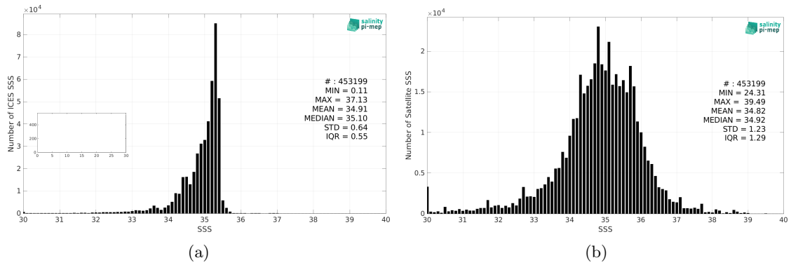
Figure 2: Histograms of SSS from ICES (a) and SMOS SSS L3 v335 - 10 Days - 25 km (CATDS-CPDC) (b) considering all match-up pairs per bins of 0.1 over the North Atlantic Ocean Pi-MEP region and for the full satellite product period.
