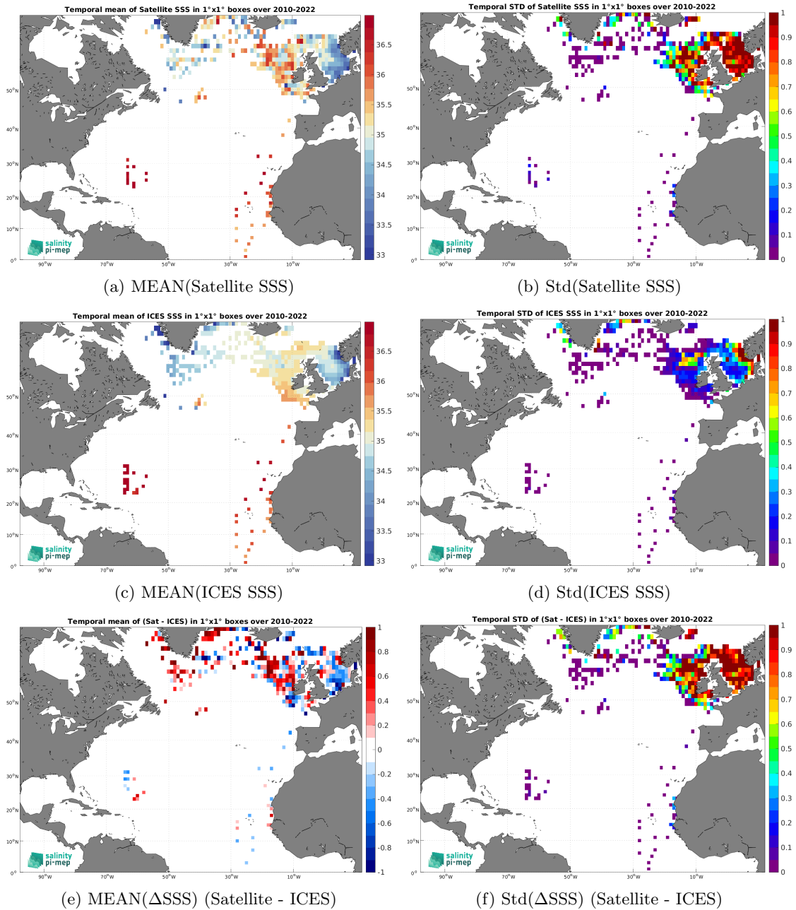
Figure 6: Temporal mean (left) and Std (right) of SSS from SMOS SSS L3 v335 - 10 Days - 25 km (CATDS-CPDC) (top), ICES (middle), and of \Delta SSS (Satellite - ICES). Only match-up pairs are used to generate these maps.
