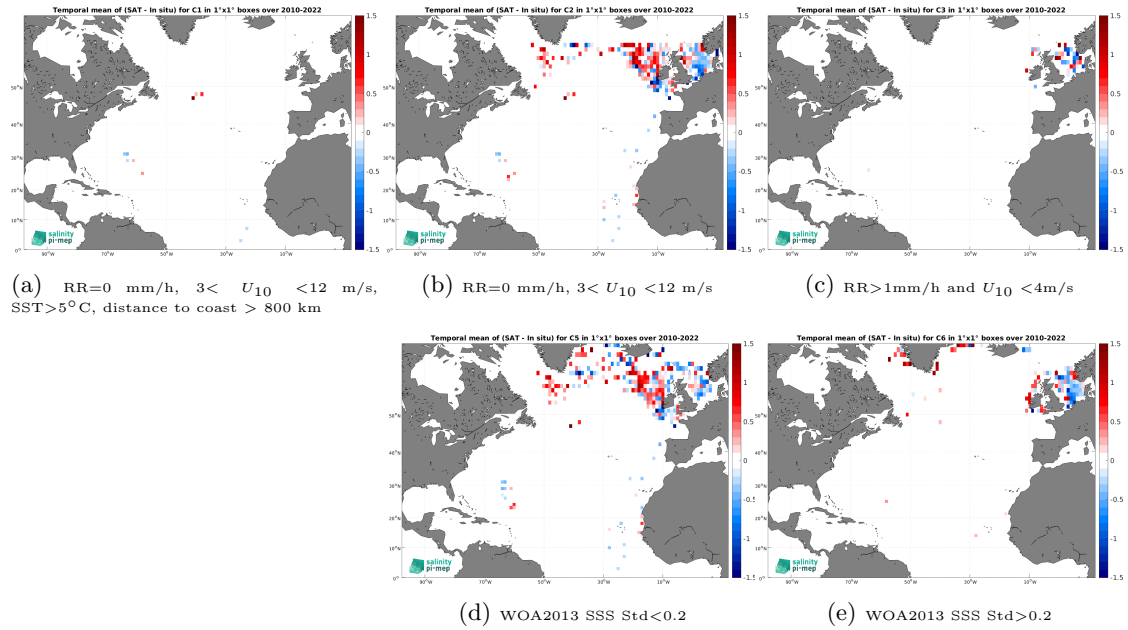
Figure 12: Temporal mean gridded over spatial boxes of size 1^\circ \times 1^\circ of \Delta\text{SSS} (SMOS SSS L3 v335 - 10 Days - 25 km (CATDS-CPDC) - ICES) for 5 different subdatasets corresponding to:RR=0 mm/h, 3 < U_{10} < 12 m/s, SST >5^\circ\text{C} , distance to coast > 800 km (a), RR=0 mm/h, 3 < U_{10} < 12 m/s (b), RR >1 mm/h and U_{10} < 4 m/s (c), WOA2013 SSS Std <0.2 (d), WOA2013 SSS Std >0.2 (e).
