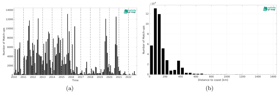
Figure 1: Number of match-ups between ICES and SMOS SSS L3 v335 - 10 Days - 25 km (CATDS-CPDC) SSS as a function of time (a) and as function of the distance to coast (b) over the North Atlantic Ocean Pi-MEP region and for the full satellite product period.
