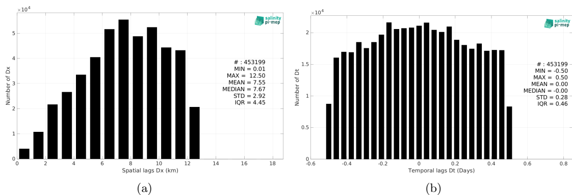
Figure 5: Histograms of the spatial (a) and temporal (b) lags between the location/time of the ICES measurement and the date of the corresponding SMOS SSS L3 v335 - 10 Days - 25 km (CATDS-CPDC) SSS pixel.
