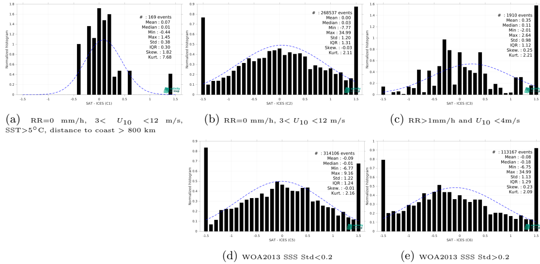
Figure 13: Normalized histogram of \Delta SSS (SMOS SSS L3 v335 - 10 Days - 25 km (CATDS-CPDC) - ICES) for 5 different subdatasets corresponding to: RR=0 mm/h, 3 < U_{10} < 12 m/s, SST > 5°C, distance to coast > 800 km (a), RR=0 mm/h, 3 < U_{10} < 12 m/s (b), RR > 1mm/h and U_{10} < 4 m/s (c), WOA2013 SSS Std < 0.2 (d), WOA2013 SSS Std > 0.2 (e).
