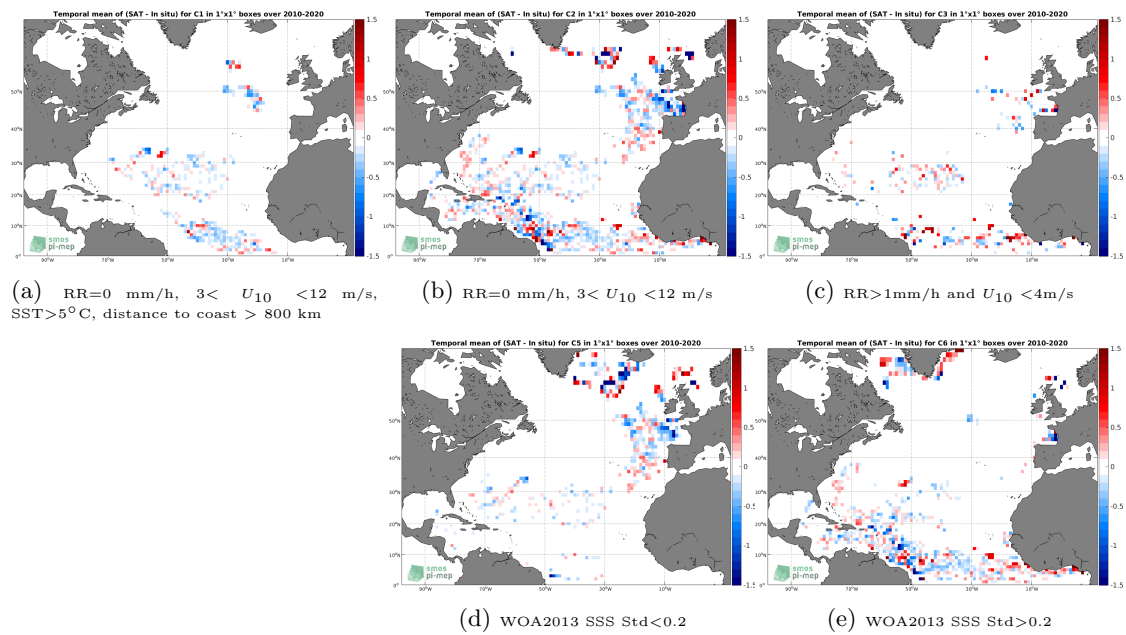
Figure 11: Temporal mean gridded over spatial boxes of size 1^\circ \times 1^\circ of \Delta\text{SSS} (SMOS SSS L3 v335 - 10 Days - 25 km (CATDS-CPDC) - Surface drifters) for 5 different subdatasets corresponding to: RR=0 mm/h, 3 < U_{10} < 12 m/s, SST > 5^\circ\text{C} , distance to coast > 800 km (a), RR=0 mm/h, 3 < U_{10} < 12 m/s (b), RR > 1 mm/h and U_{10} < 4 m/s (c), WOA2013 SSS Std < 0.2 (d), WOA2013 SSS Std > 0.2 (e).
