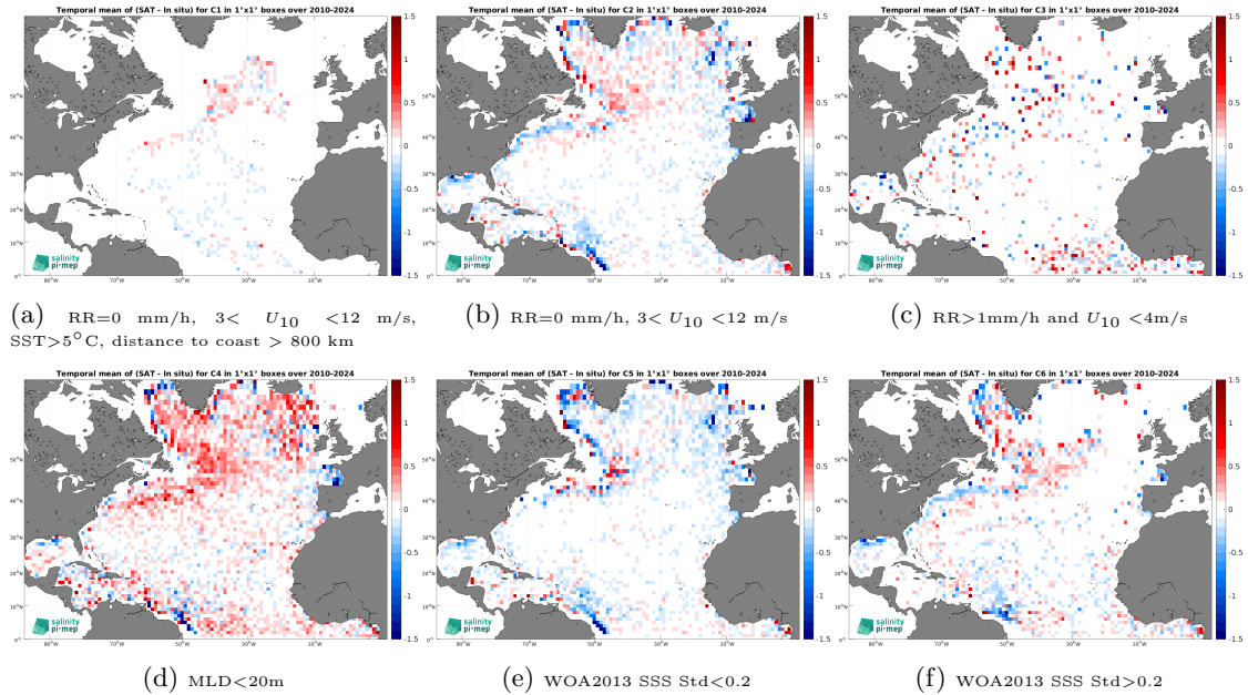
Figure 14: Temporal mean gridded over spatial boxes of size 1^\circ \times 1^\circ of \Delta\text{SSS} (SMOS SSS L3 v335 - 10 Days - 25 km (CATDS-CPDC) - Argo) for 6 different subdatasets corresponding to:RR=0 mm/h, 3 < U_{10} < 12 m/s, SST>5°C, distance to coast > 800 km (a), RR=0 mm/h, 3 < U_{10} < 12 m/s (b), RR>1mm/h and U_{10} < 4 m/s (c),MLD<20m (d),WOA2013 SSS Std<0.2 (e),WOA2013 SSS Std>0.2 (f).
