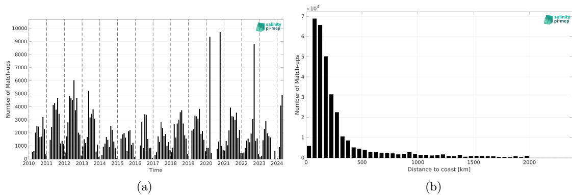
Figure 2: Number of match-ups between TSG (SAMOS) and SMOS SSS L2Q v333 - 0.25 Deg (CATDS-CPDC) SSS as a function of time (a) and as function of the distance to coast (b) over the North Atlantic Ocean Pi-MEP region and for the full satellite product period.
