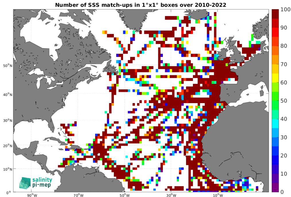
Figure 5: Number of SSS match-ups between TSG (GOSUD-Research-vessel) SSS and the SMOS SSS L2Q v333 - 0.25 Deg (CATDS-CPDC) SSS product for the North Atlantic Ocean Pi-MEP region over 1°×1° boxes and for the full satellite product period.
