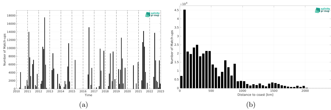
Figure 2: Number of match-ups between TSG (CSIC-UTM) and SMOS SSS L2Q v333 - 0.25 Deg (CATDS-CPDC) SSS as a function of time (a) and as function of the distance to coast (b) over the North Atlantic Ocean Pi-MEP region and for the full satellite product period.
