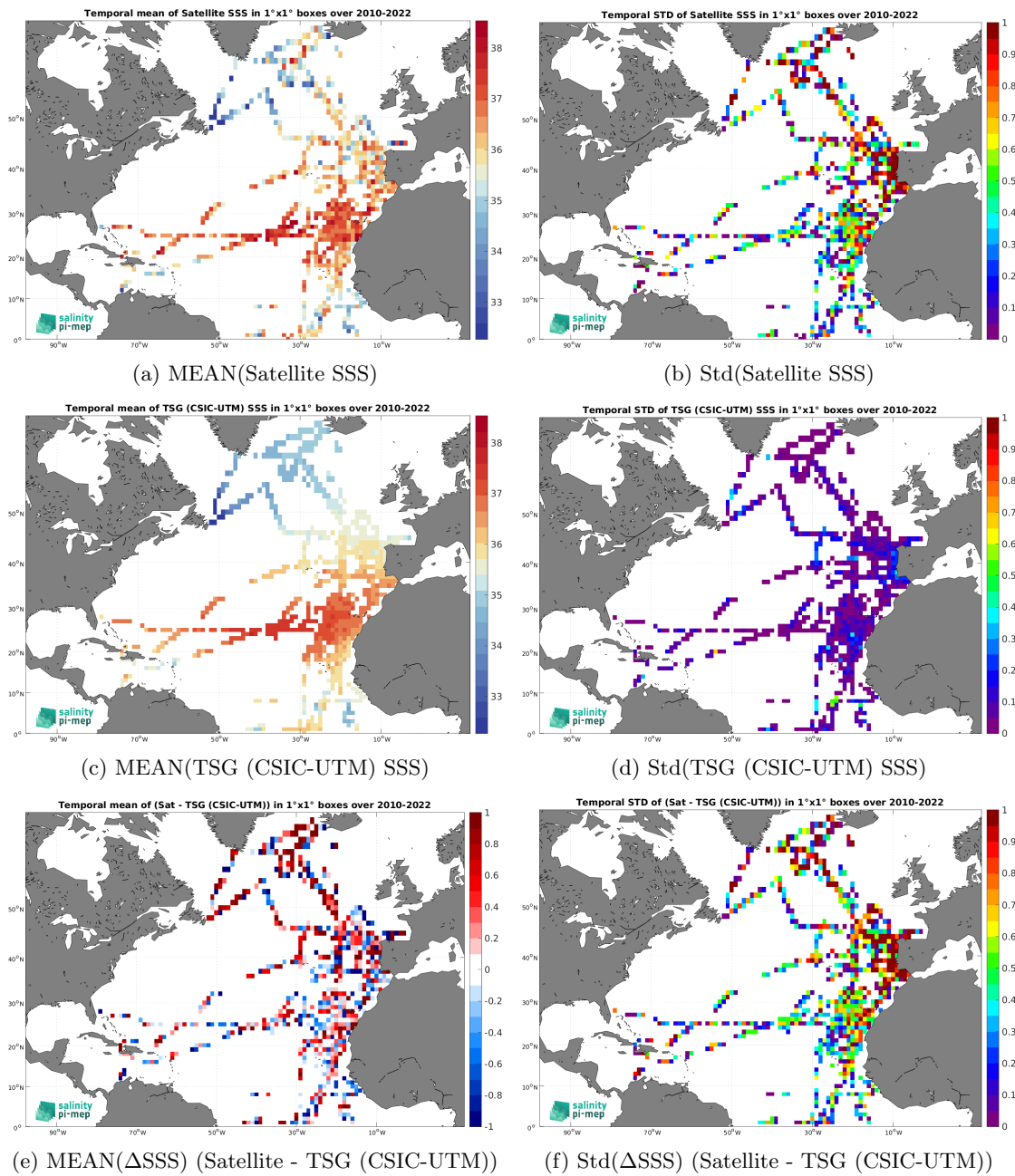
Figure 7: Temporal mean (left) and Std (right) of SSS from SMOS SSS L2Q v333 - 0.25 Deg (CATDS-CPDC) (top), TSG (CSIC-UTM) (middle), and of \Delta SSS (Satellite - TSG (CSIC-UTM)). Only match-up pairs are used to generate these maps.
