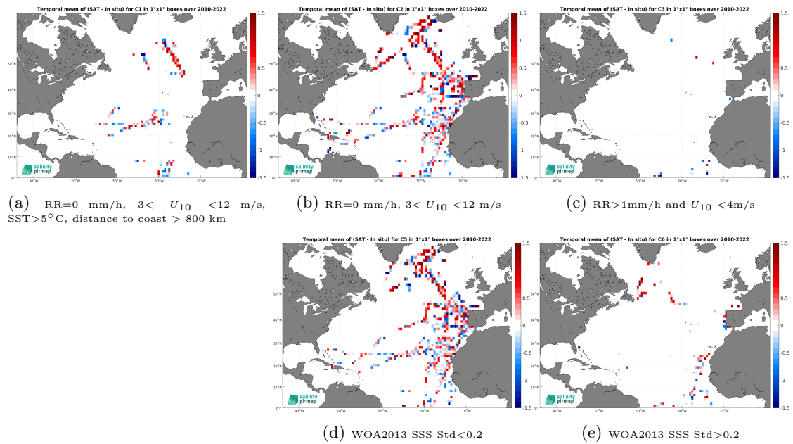
Figure 14: Temporal mean gridded over spatial boxes of size 1^\circ \times 1^\circ of \Delta\text{SSS} (SMOS SSS L2Q v333 - 0.25 Deg (CATDS-CPDC) - TSG (CSIC-UTM)) for 5 different subdatasets corresponding to:RR=0 mm/h, 3 < U_{10} < 12 m/s, SST > 5°C, distance to coast > 800 km (a), RR=0 mm/h, 3 < U_{10} < 12 m/s (b), RR > 1mm/h and U_{10} < 4 m/s (c), WOA2013 SSS Std < 0.2 (d), WOA2013 SSS Std > 0.2 (e).
