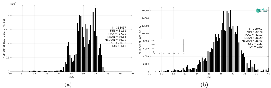
Figure 3: Histograms of SSS from TSG (CSIC-UTM) (a) and SMOS SSS L2Q v333 - 0.25 Deg (CATDS-CPDC) (b) considering all match-up pairs per bins of 0.1 over the North Atlantic Ocean Pi-MEP region and for the full satellite product period.
