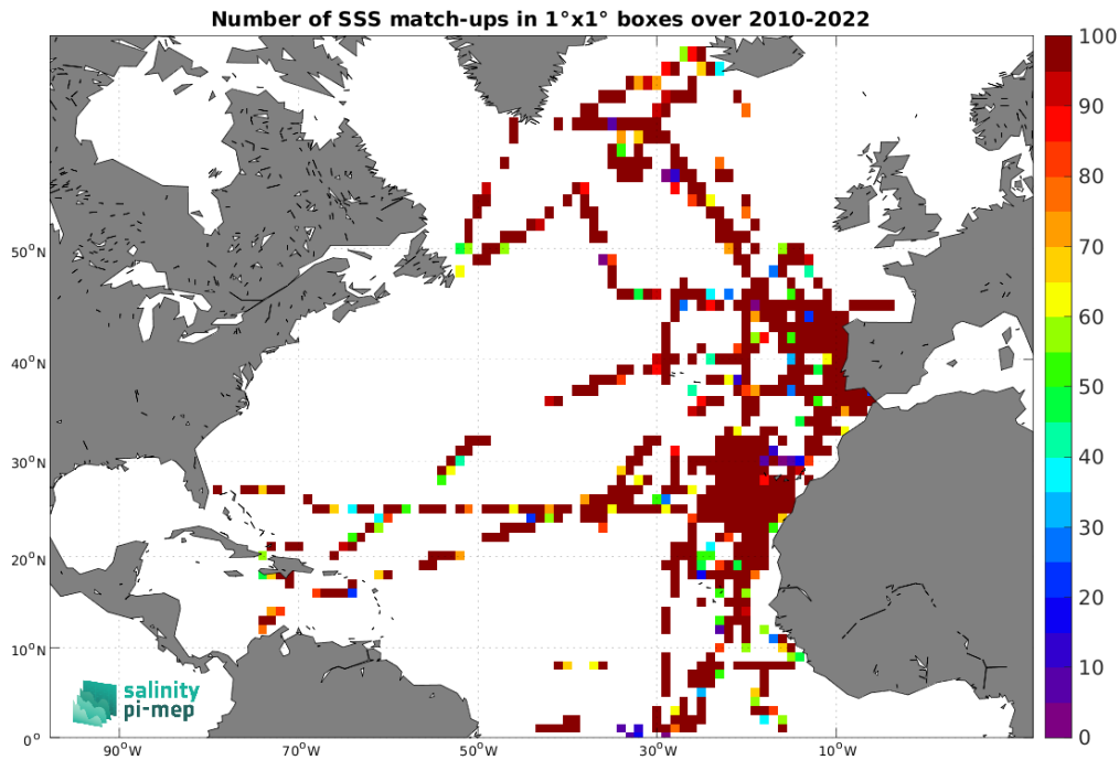
Figure 5: Number of SSS match-ups between TSG (CSIC-UTM) SSS and the SMOS SSS L2Q v333 - 0.25 Deg (CATDS-CPDC) SSS product for the North Atlantic Ocean Pi-MEP region over 1^\circ \times 1^\circ boxes and for the full satellite product period.
