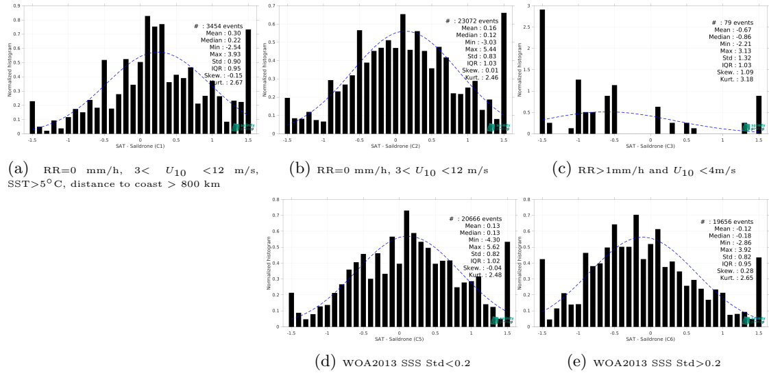
Figure 15: Normalized histogram of \Delta SSS (SMOS SSS L2Q v333 - 0.25 Deg (CATDS-CPDC) - Saldrone) for 5 different subdatasets corresponding to: RR=0 mm/h, 3 < U_{10} < 12 m/s, SST > 5°C, distance to coast > 800 km (a), RR=0 mm/h, 3 < U_{10} < 12 m/s (b), RR > 1mm/h and U_{10} < 4 m/s (c), WOA2013 SSS Std < 0.2 (d), WOA2013 SSS Std > 0.2 (e).
