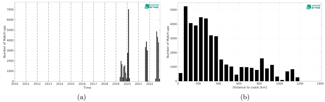
Figure 2: Number of match-ups between Saildrone and SMOS SSS L2Q v333 - 0.25 Deg (CATDS-CPDC) SSS as a function of time (a) and as function of the distance to the coast (b) over the North Atlantic Ocean Pi-MEP region and for the full satellite product period.
