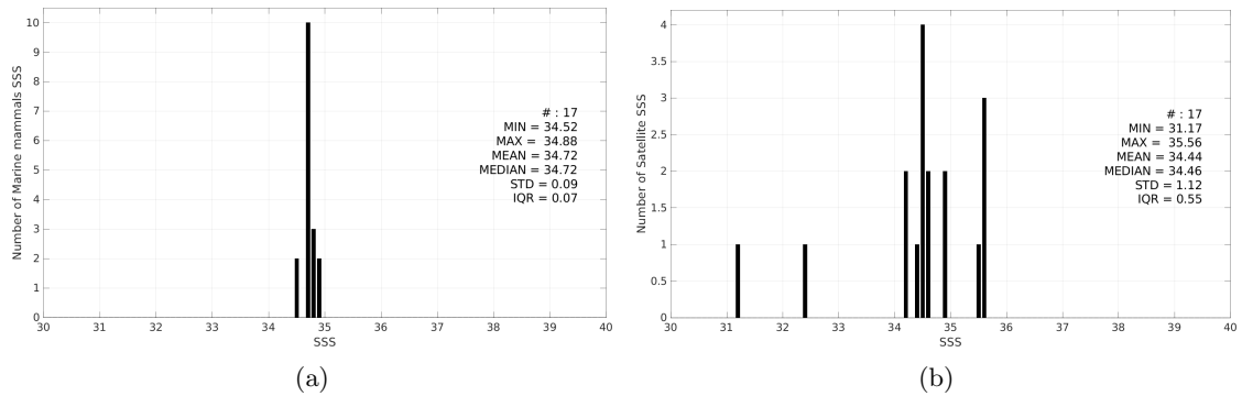
Figure 3: Histograms of SSS from Marine mammals (a) and SMOS SSS L2Q v333 - 0.25 Deg (CATDS-CPDC) (b) considering all match-up pairs per bins of 0.1 over the North Atlantic Ocean Pi-MEP region and for the full satellite product period.
