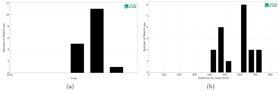
Figure 2: Number of match-ups between Marine mammals and SMOS SSS L2Q v333 - 0.25 Deg (CATDS-CPDC) SSS as a function of time (a) and as function of the distance to coast (b) over the North Atlantic Ocean Pi-MEP region and for the full satellite product period.
