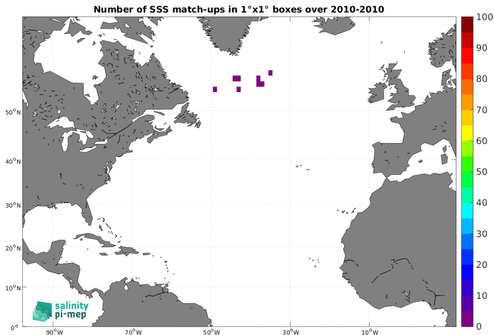
Figure 5: Number of SSS match-ups between Marine mammals SSS and the SMOS SSS L2Q v333 - 0.25 Deg (CATDS-CPDC) SSS product for the North Atlantic Ocean Pi-MEP region over 1^\circ \times 1^\circ boxes and for the full satellite product period.
