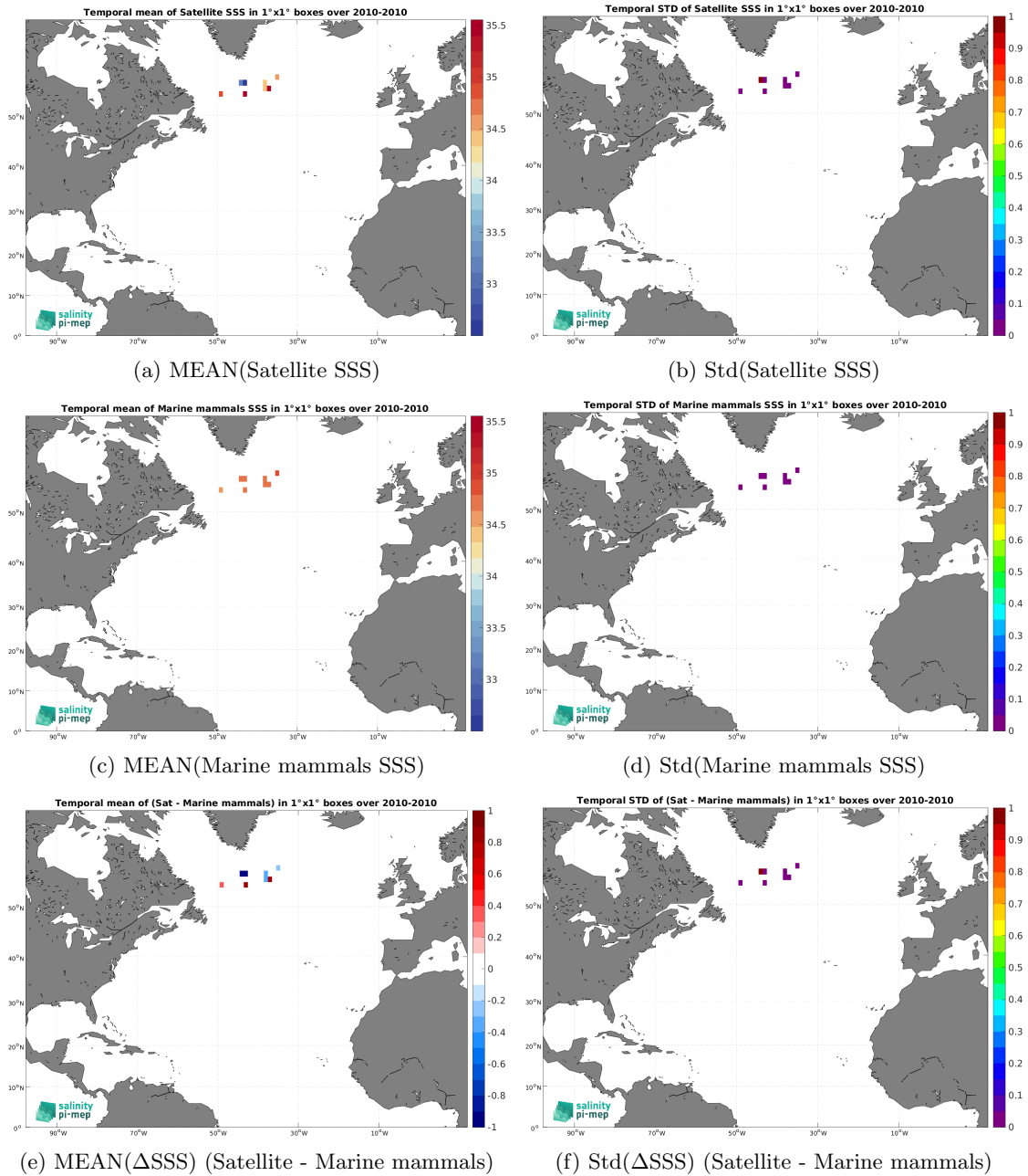
Figure 7: Temporal mean (left) and Std (right) of SSS from SMOS SSS L2Q v333 - 0.25 Deg (CATDS-CPDC) (top), Marine mammals (middle), and of \Delta SSS (Satellite - Marine mammals). Only match-up pairs are used to generate these maps.
