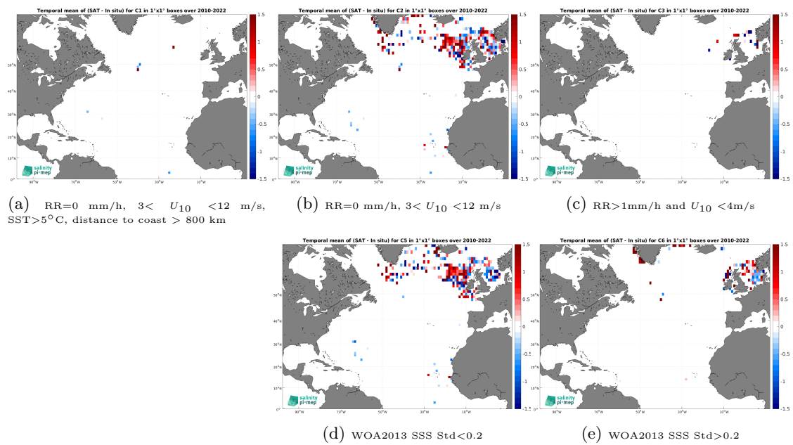
Figure 14: Temporal mean gridded over spatial boxes of size 1^\circ \times 1^\circ of \Delta\text{SSS} (SMOS SSS L2Q v333 - 0.25 Deg (CATDS-CPDC) - ICES) for 5 different subdatasets corresponding to:RR=0 mm/h, 3 < U_{10} < 12 m/s, SST > 5°C, distance to coast > 800 km (a), RR=0 mm/h, 3 < U_{10} < 12 m/s (b), RR > 1mm/h and U_{10} < 4 m/s (c), WOA2013 SSS Std < 0.2 (d), WOA2013 SSS Std > 0.2 (e).
