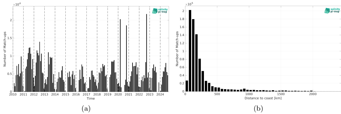
Figure 2: Number of match-ups between TSG (SAMOS) and SMOS SSS L3 v332 - 9 Days (CATDS-CPDC) SSS as a function of time (a) and as function of the distance to coast (b) over the North Atlantic Ocean Pi-MEP region and for the full satellite product period.
