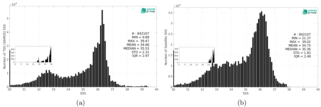
Figure 3: Histograms of SSS from TSG (SAMOS) (a) and SMOS SSS L3 v332 - 9 Days (CATDS-CPDC) (b) considering all match-up pairs per bins of 0.1 over the North Atlantic Ocean Pi-MEP region and for the full satellite product period.
