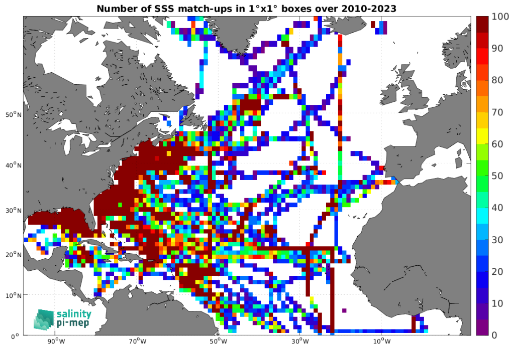
Figure 4: Number of SSS match-ups between TSG (SAMOS) SSS and the SMOS SSS L3 v332 - 9 Days (CATDS-CPDC) SSS product for the North Atlantic Ocean Pi-MEP region over 1^\circ \times 1^\circ boxes and for the full satellite product period.
