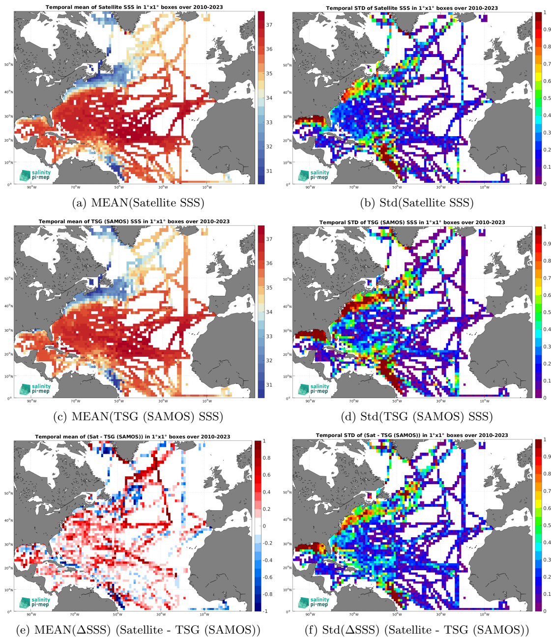
Figure 6: Temporal mean (left) and Std (right) of SSS from SMOS SSS L3 v332 - 9 Days (CATDS-CPDC) (top), TSG (SAMOS) (middle), and of \Delta SSS (Satellite - TSG (SAMOS)). Only match-up pairs are used to generate these maps.
