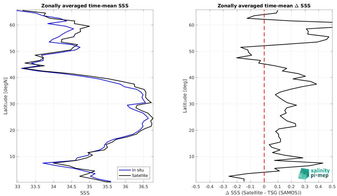
Figure 8: Left panel: Zonal mean SSS from SMOS SSS L3 v332 - 9 Days (CATDS-CPDC) satellite product (black) and from TSG (SAMOS) (blue). Right panel: Zonal mean of \Delta SSS (Satellite - TSG (SAMOS)) for all the collected Pi-MEP match-up pairs estimated over the full satellite product period.
