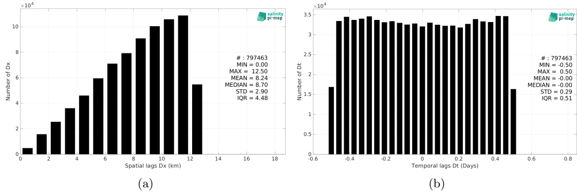
Figure 5: Histograms of the spatial (a) and temporal (b) lags between the location/time of the TSG (SAMOS) measurement and the date of the corresponding SMOS SSS L3 v332 - 9 Days (CATDS-CPDC) SSS pixel.
