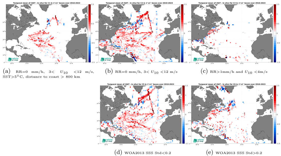
Figure 12: Temporal mean gridded over spatial boxes of size 1^\circ \times 1^\circ of \Delta\text{SSS} (SMOS SSS L3 v332 - 9 Days (CATDS-CPDC) - TSG (SAMOS)) for 5 different subdatasets corresponding to:RR=0 mm/h, 3 < U_{10} < 12 m/s, SST > 5^\circ\text{C} , distance to coast > 800 km (a), RR=0 mm/h, 3 < U_{10} < 12 m/s (b), RR > 1 mm/h and U_{10} < 4 m/s (c), WOA2013 SSS Std < 0.2 (d), WOA2013 SSS Std > 0.2 (e).
