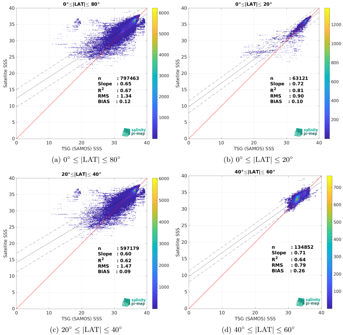
Figure 9: Contour maps of the concentration of SMOS SSS L3 v332 - 9 Days (CATDS-CPDC) SSS (y-axis) versus TSG (SAMOS) SSS (x-axis) at match-up pairs for different latitude bands. For each plot, the red line shows x=y . The black thin and dashed lines indicate a linear fit through the data cloud and the \pm 95\% confidence levels, respectively. The number match-up pairs n , the slope and R^2 coefficient of the linear fit, the root mean square (RMS) and the mean bias between satellite and in situ data are indicated for each latitude band in each plots.
