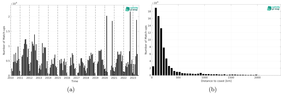
Figure 1: Number of match-ups between TSG (SAMOS) and SMOS SSS L3 v332 - 9 Days (CATDS-CPDC) SSS as a function of time (a) and as function of the distance to coast (b) over the North Atlantic Ocean Pi-MEP region and for the full satellite product period.
