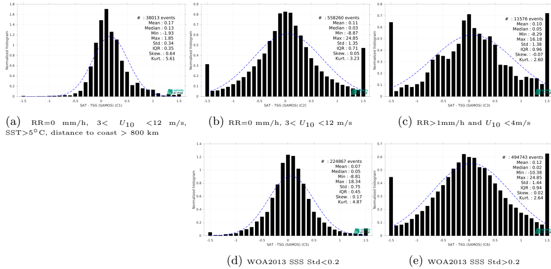
Figure 13: Normalized histogram of \Delta SSS (SMOS SSS L3 v332 - 9 Days (CATDS-CPDC) - TSG (SAMOS)) for 5 different subdatasets corresponding to: RR=0 mm/h, 3 < U_{10} < 12 m/s, SST>5°C, distance to coast > 800 km (a), RR=0 mm/h, 3 < U_{10} < 12 m/s (b), RR>1mm/h and U_{10} < 4 m/s (c), WOA2013 SSS Std<0.2 (d), WOA2013 SSS Std>0.2 (e).
