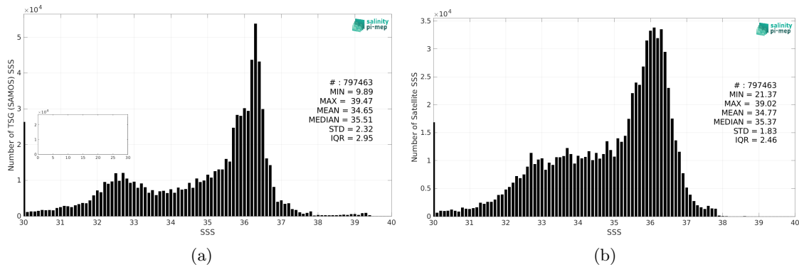
Figure 2: Histograms of SSS from TSG (SAMOS) (a) and SMOS SSS L3 v332 - 9 Days (CATDS-CPDC) (b) considering all match-up pairs per bins of 0.1 over the North Atlantic Ocean Pi-MEP region and for the full satellite product period.
