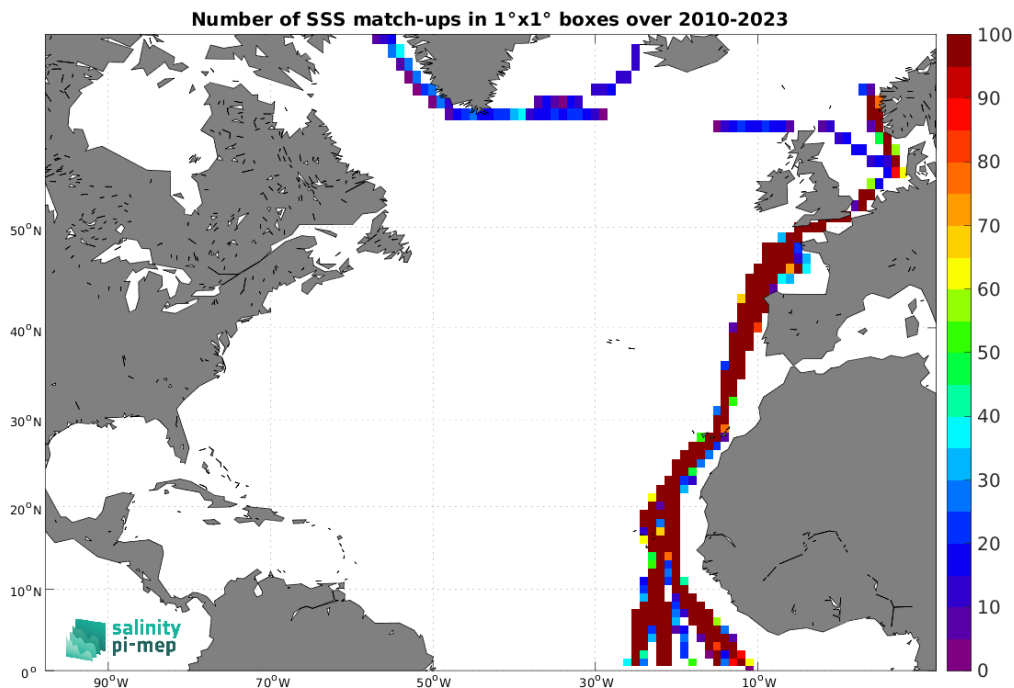
Figure 5: Number of SSS match-ups between TSG (Polarstern) SSS and the SMOS SSS L3 v332 - 9 Days (CATDS-CPDC) SSS product for the North Atlantic Ocean Pi-MEP region over 1^\circ \times 1^\circ boxes and for the full satellite product period.
