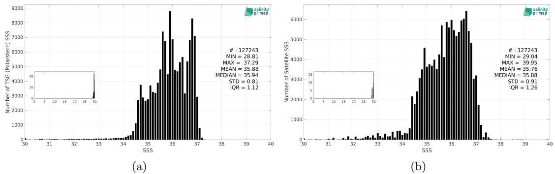
Figure 3: Histograms of SSS from TSG (Polarstern) (a) and SMOS SSS L3 v332 - 9 Days (CATDS-CPDC) (b) considering all match-up pairs per bins of 0.1 over the North Atlantic Ocean Pi-MEP region and for the full satellite product period.
