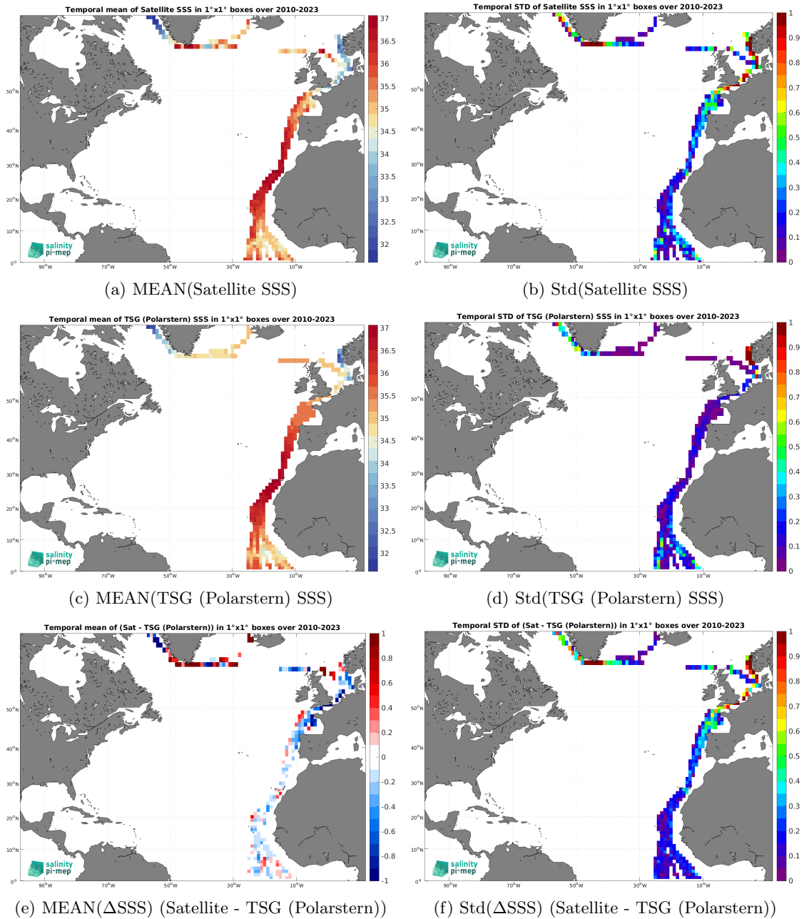
Figure 7: Temporal mean (left) and Std (right) of SSS from SMOS SSS L3 v332 - 9 Days (CATDS-CPDC) (top), TSG (Polarstern) (middle), and of \Delta SSS (Satellite - TSG (Polarstern)). Only match-up pairs are used to generate these maps.
