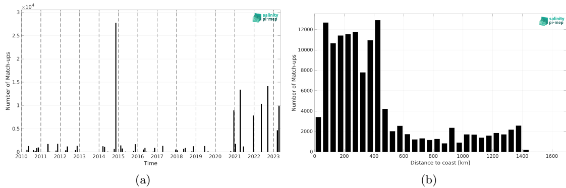
Figure 2: Number of match-ups between TSG (Polarstern) and SMOS SSS L3 v332 - 9 Days (CATDS-CPDC) SSS as a function of time (a) and as function of the distance to coast (b) over the North Atlantic Ocean Pi-MEP region and for the full satellite product period.
