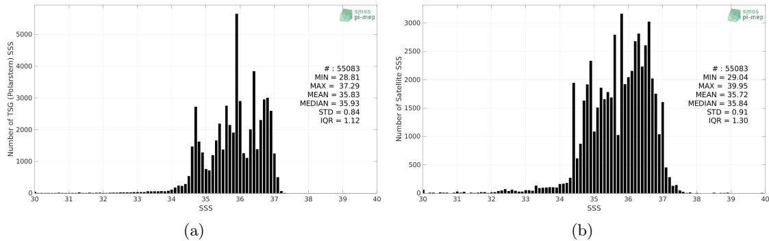
Figure 2: Histograms of SSS from TSG (Polarstern) (a) and SMOS SSS L3 v332 - 9 Days (CATDS-CPDC) (b) considering all match-up pairs per bins of 0.1 over the North Atlantic Ocean Pi-MEP region and for the full satellite product period.
