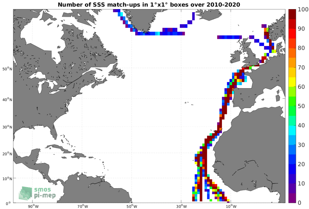
Figure 4: Number of SSS match-ups between TSG (Polarstern) SSS and the SMOS SSS L3 v332 - 9 Days (CATDS-CPDC) SSS product for the North Atlantic Ocean Pi-MEP region over 1^\circ \times 1^\circ boxes and for the full satellite product period.
