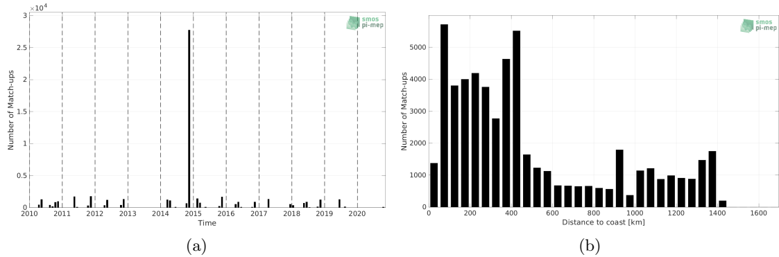
Figure 1: Number of match-ups between TSG (Polarstern) and SMOS SSS L3 v332 - 9 Days (CATDS-CPDC) SSS as a function of time (a) and as function of the distance to coast (b) over the North Atlantic Ocean Pi-MEP region and for the full satellite product period.
