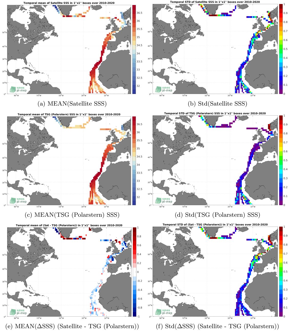
Figure 6: Temporal mean (left) and Std (right) of SSS from SMOS SSS L3 v332 - 9 Days (CATDS-CPDC) (top), TSG (Polarstern) (middle), and of \Delta SSS (Satellite - TSG (Polarstern)). Only match-up pairs are used to generate these maps.
