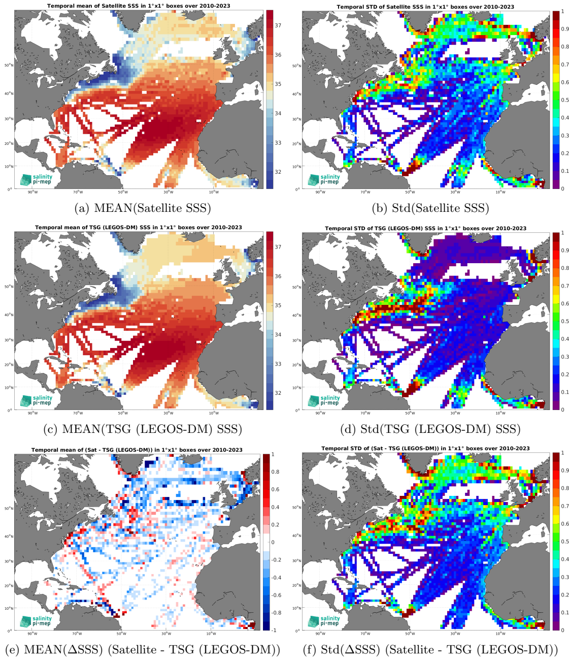
Figure 7: Temporal mean (left) and Std (right) of SSS from SMOS SSS L3 v332 - 9 Days (CATDS-CPDC) (top), TSG (LEGOS-DM) (middle), and of \Delta SSS (Satellite - TSG (LEGOS-DM)). Only match-up pairs are used to generate these maps.
