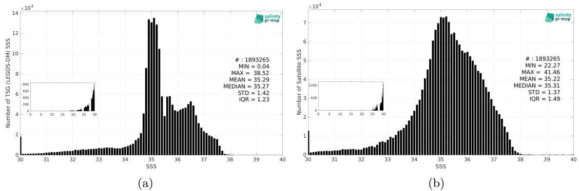
Figure 3: Histograms of SSS from TSG (LEGOS-DM) (a) and SMOS SSS L3 v332 - 9 Days (CATDS-CPDC) (b) considering all match-up pairs per bins of 0.1 over the North Atlantic Ocean Pi-MEP region and for the full satellite product period.
