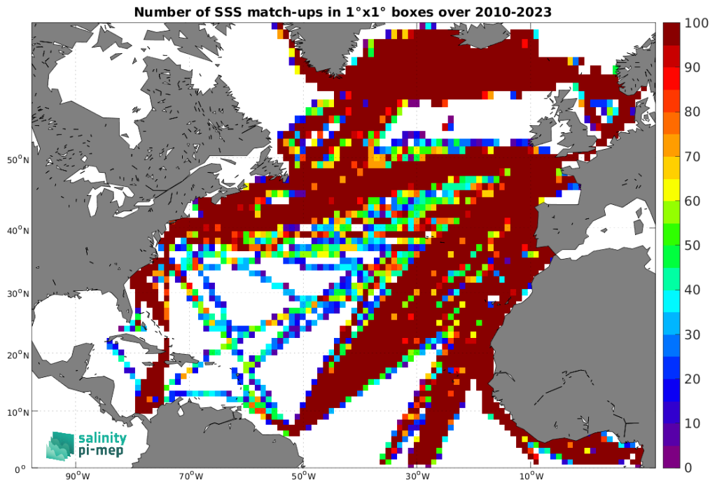
Figure 5: Number of SSS match-ups between TSG (LEGOS-DM) SSS and the SMOS SSS L3 v332 - 9 Days (CATDS-CPDC) SSS product for the North Atlantic Ocean Pi-MEP region over 1^\circ \times 1^\circ boxes and for the full satellite product period.
