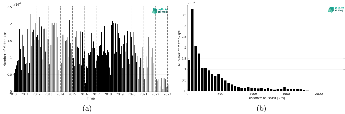
Figure 2: Number of match-ups between TSG (LEGOS-DM) and SMOS SSS L3 v332 - 9 Days (CATDS-CPDC) SSS as a function of time (a) and as function of the distance to coast (b) over the North Atlantic Ocean Pi-MEP region and for the full satellite product period.
