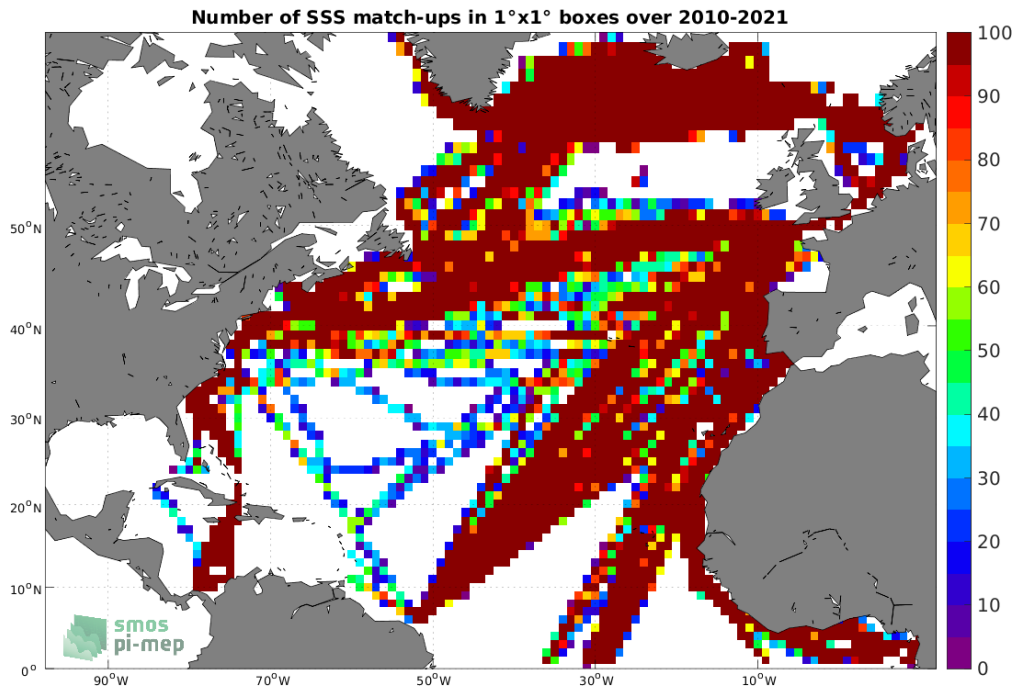
Figure 4: Number of SSS match-ups between TSG (LEGOS-DM) SSS and the SMOS SSS L3 v332 - 9 Days (CATDS-CPDC) SSS product for the North Atlantic Ocean Pi-MEP region over 1^\circ \times 1^\circ boxes and for the full satellite product period.
