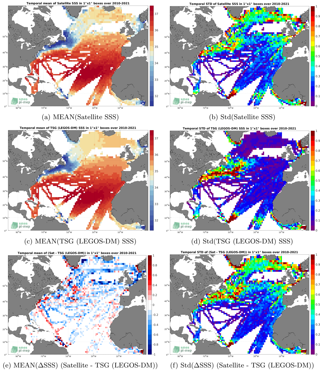
Figure 6: Temporal mean (left) and Std (right) of SSS from SMOS SSS L3 v332 - 9 Days (CATDS-CPDC) (top), TSG (LEGOS-DM) (middle), and of \Delta SSS (Satellite - TSG (LEGOS-DM)). Only match-up pairs are used to generate these maps.
