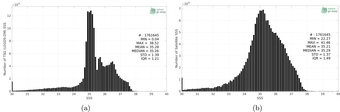
Figure 2: Histograms of SSS from TSG (LEGOS-DM) (a) and SMOS SSS L3 v332 - 9 Days (CATDS-CPDC) (b) considering all match-up pairs per bins of 0.1 over the North Atlantic Ocean Pi-MEP region and for the full satellite product period.
