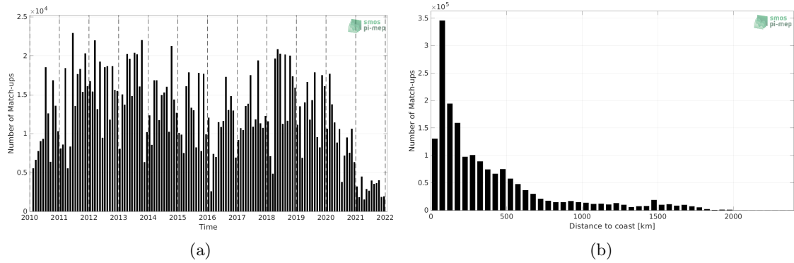
Figure 1: Number of match-ups between TSG (LEGOS-DM) and SMOS SSS L3 v332 - 9 Days (CATDS-CPDC) SSS as a function of time (a) and as function of the distance to coast (b) over the North Atlantic Ocean Pi-MEP region and for the full satellite product period.
