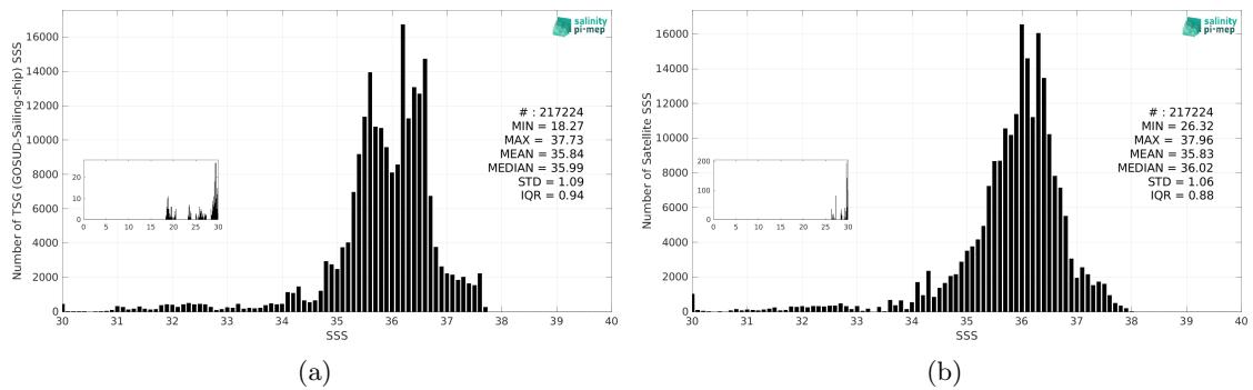
Figure 3: Histograms of SSS from TSG (GOSUD-Sailing-ship) (a) and SMOS SSS L3 v332 - 9 Days (CATDS-CPDC) (b) considering all match-up pairs per bins of 0.1 over the North Atlantic Ocean Pi-MEP region and for the full satellite product period.
