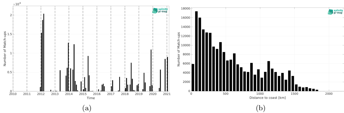
Figure 2: Number of match-ups between TSG (GOSUD-Sailing-ship) and SMOS SSS L3 v332 - 9 Days (CATDS-CPDC) SSS as a function of time (a) and as function of the distance to coast (b) over the North Atlantic Ocean Pi-MEP region and for the full satellite product period.
