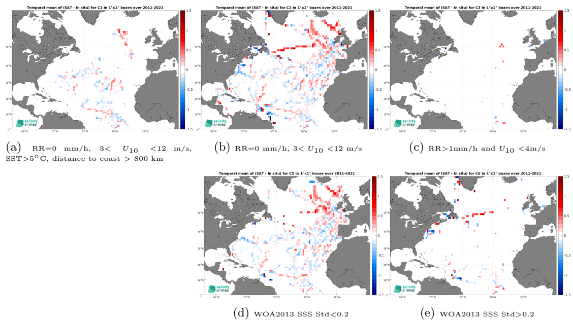
Figure 14: Temporal mean gridded over spatial boxes of size 1^\circ \times 1^\circ of \Delta\text{SSS} (SMOS SSS L3 v332 - 9 Days (CATDS-CPDC) - TSG (GOSUD-Sailing-ship)) for 5 different subdatasets corresponding to:RR=0 mm/h, 3 < U_{10} < 12 m/s, SST > 5°C, distance to coast > 800 km (a), RR=0 mm/h, 3 < U_{10} < 12 m/s (b), RR > 1mm/h and U_{10} < 4 m/s (c), WOA2013 SSS Std < 0.2 (d), WOA2013 SSS Std > 0.2 (e).
