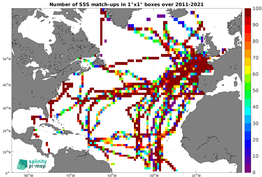
Figure 5: Number of SSS match-ups between TSG (GOSUD-Sailing-ship) SSS and the SMOS SSS L3 v332 - 9 Days (CATDS-CPDC) SSS product for the North Atlantic Ocean Pi-MEP region over 1°×1° boxes and for the full satellite product period.
