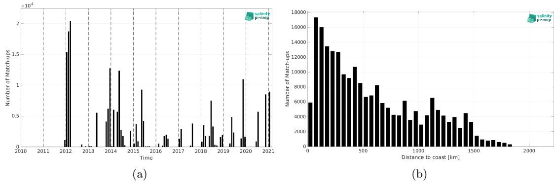
Figure 1: Number of match-ups between TSG (GOSUD-Sailing-ship) and SMOS SSS L3 v332 - 9 Days (CATDS-CPDC) SSS as a function of time (a) and as function of the distance to coast (b) over the North Atlantic Ocean Pi-MEP region and for the full satellite product period.
