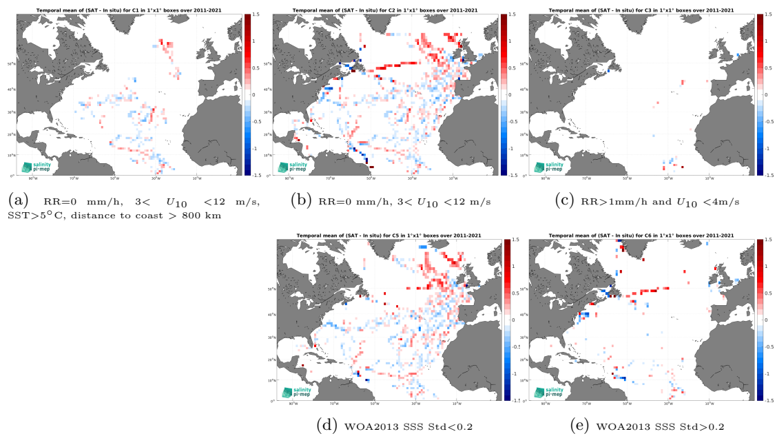
Figure 12: Temporal mean gridded over spatial boxes of size 1^\circ \times 1^\circ of \Delta\text{SSS} (SMOS SSS L3 v332 - 9 Days (CATDS-CPDC) - TSG (GOSUD-Sailing-ship)) for 5 different subdatasets corresponding to:RR=0 mm/h, 3 < U_{10} < 12 m/s, SST>5°C, distance to coast > 800 km (a), RR=0 mm/h, 3 < U_{10} < 12 m/s (b), RR>1mm/h and U_{10} < 4 m/s (c), WOA2013 SSS Std<0.2 (d), WOA2013 SSS Std>0.2 (e).
