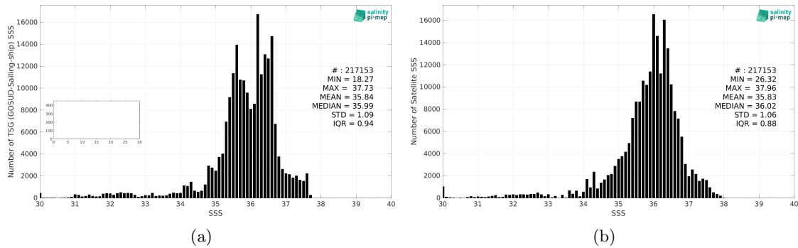
Figure 2: Histograms of SSS from TSG (GOSUD-Sailing-ship) (a) and SMOS SSS L3 v332 - 9 Days (CATDS-CPDC) (b) considering all match-up pairs per bins of 0.1 over the North Atlantic Ocean Pi-MEP region and for the full satellite product period.
