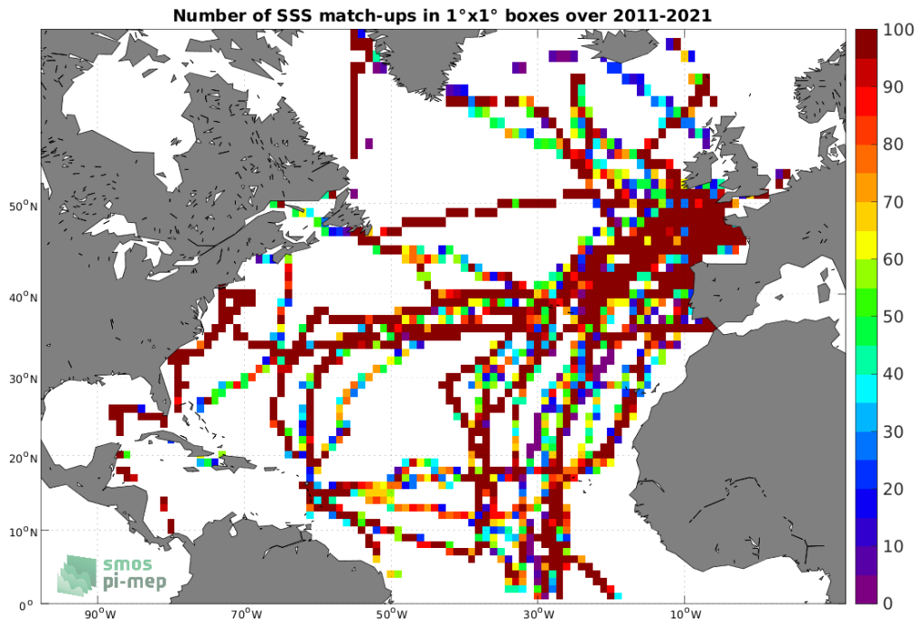
Figure 4: Number of SSS match-ups between TSG (GOSUD-Sailing-ship) SSS and the SMOS SSS L3 v332 - 9 Days (CATDS-CPDC) SSS product for the North Atlantic Ocean Pi-MEP region over 1°x1° boxes and for the full satellite product period.
