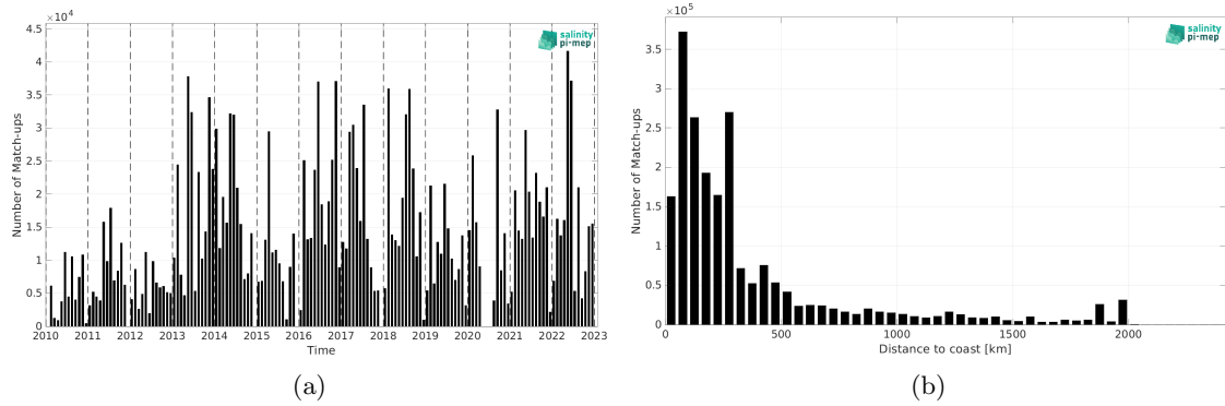
Figure 2: Number of match-ups between TSG (GOSUD-Research-vessel) and SMOS SSS L3 v332 - 9 Days (CATDS-CPDC) SSS as a function of time (a) and as function of the distance to coast (b) over the North Atlantic Ocean Pi-MEP region and for the full satellite product period.
