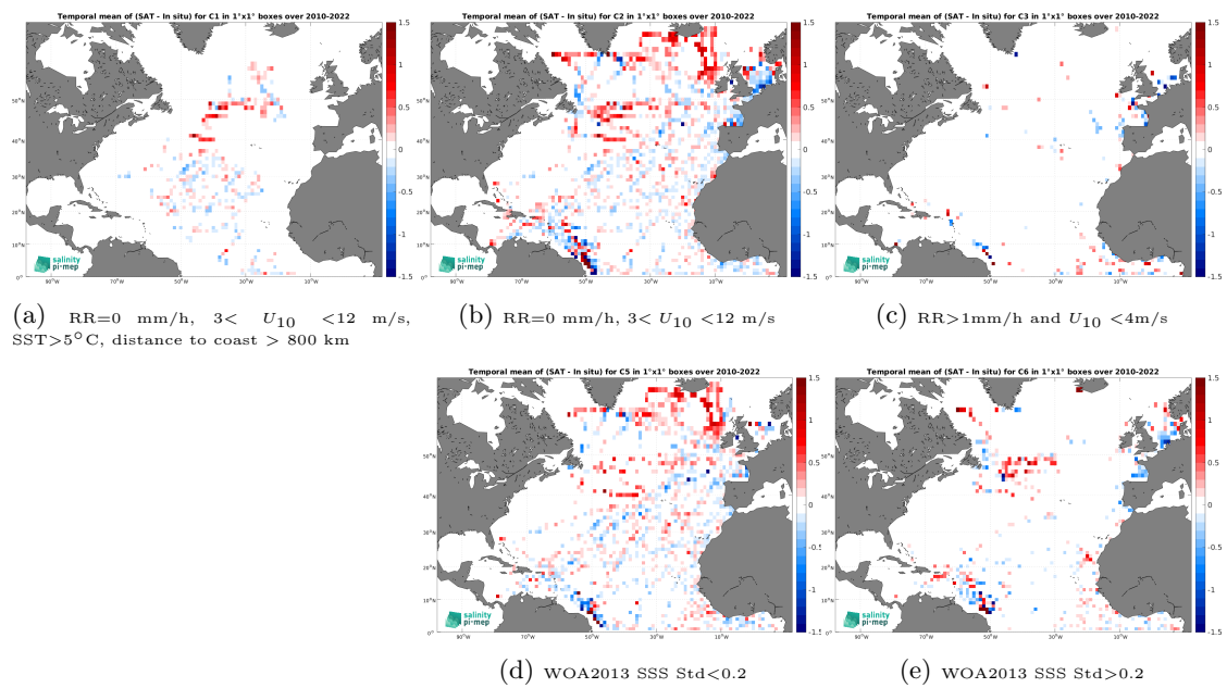
Figure 14: Temporal mean gridded over spatial boxes of size 1^\circ \times 1^\circ of \Delta\text{SSS} (SMOS SSS L3 v332 - 9 Days (CATDS-CPDC) - TSG (GOSUD-Research-vessel)) for 5 different subdatasets corresponding to:RR=0 mm/h, 3 < U_{10} < 12 m/s, SST >5^\circ\text{C} , distance to coast > 800 km (a), RR=0 mm/h, 3 < U_{10} < 12 m/s (b), RR >1 mm/h and U_{10} < 4 m/s (c), WOA2013 SSS Std <0.2 (d), WOA2013 SSS Std >0.2 (e).
