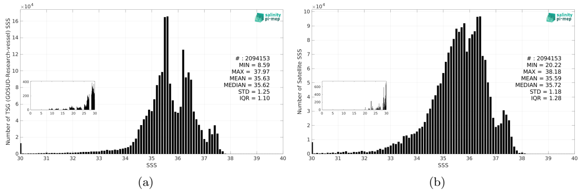
Figure 3: Histograms of SSS from TSG (GOSUD-Research-vessel) (a) and SMOS SSS L3 v332 - 9 Days (CATDS-CPDC) (b) considering all match-up pairs per bins of 0.1 over the North Atlantic Ocean Pi-MEP region and for the full satellite product period.
