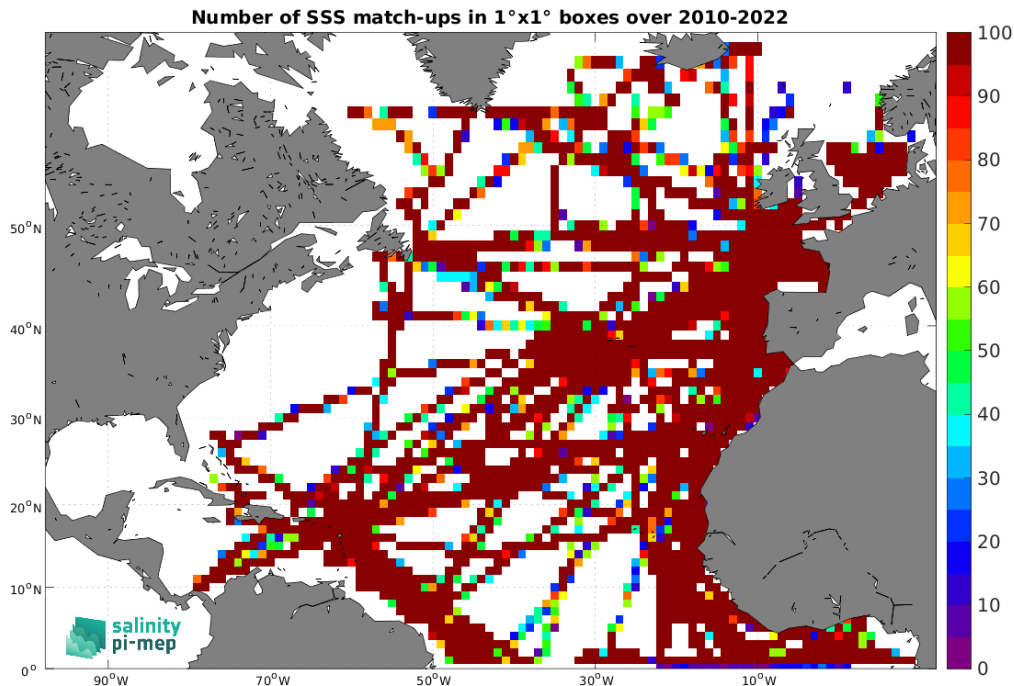
Figure 5: Number of SSS match-ups between TSG (GOSUD-Research-vessel) SSS and the SMOS SSS L3 v332 - 9 Days (CATDS-CPDC) SSS product for the North Atlantic Ocean Pi-MEP region over 1^\circ \times 1^\circ boxes and for the full satellite product period.
