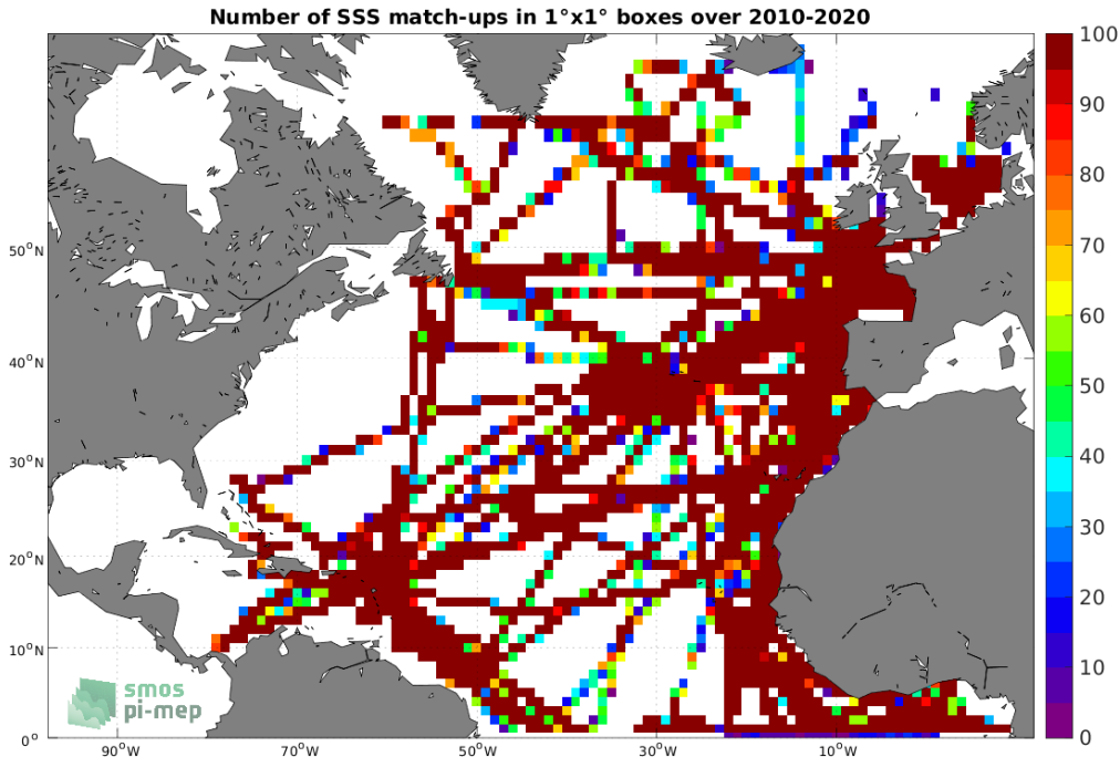
Figure 4: Number of SSS match-ups between TSG (GOSUD-Research-vessel) SSS and the SMOS SSS L3 v332 - 9 Days (CATDS-CPDC) SSS product for the North Atlantic Ocean Pi-MEP region over 1^\circ \times 1^\circ boxes and for the full satellite product period.
