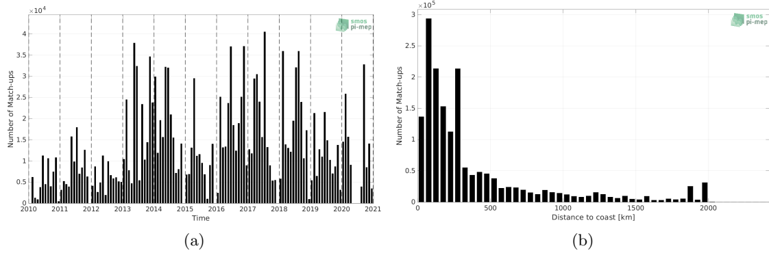
Figure 1: Number of match-ups between TSG (GOSUD-Research-vessel) and SMOS SSS L3 v332 - 9 Days (CATDS-CPDC) SSS as a function of time (a) and as function of the distance to coast (b) over the North Atlantic Ocean Pi-MEP region and for the full satellite product period.
