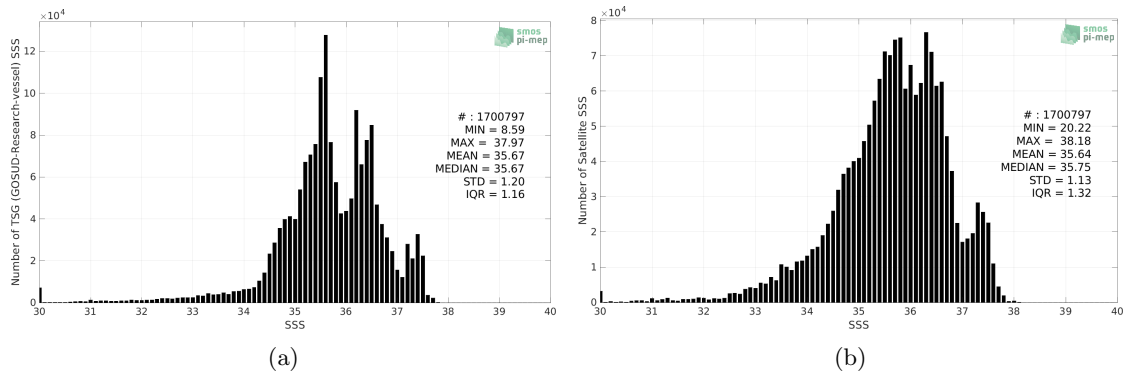
Figure 2: Histograms of SSS from TSG (GOSUD-Research-vessel) (a) and SMOS SSS L3 v332 - 9 Days (CATDS-CPDC) (b) considering all match-up pairs per bins of 0.1 over the North Atlantic Ocean Pi-MEP region and for the full satellite product period.
