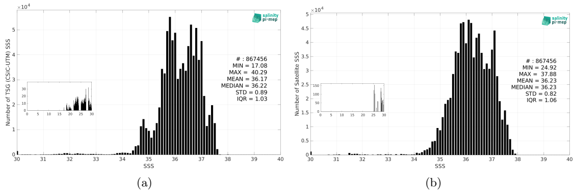
Figure 3: Histograms of SSS from TSG (CSIC-UTM) (a) and SMOS SSS L3 v332 - 9 Days (CATDS-CPDC) (b) considering all match-up pairs per bins of 0.1 over the North Atlantic Ocean Pi-MEP region and for the full satellite product period.
