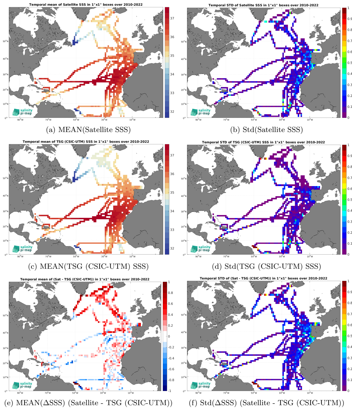
Figure 7: Temporal mean (left) and Std (right) of SSS from SMOS SSS L3 v332 - 9 Days (CATDS-CPDC) (top), TSG (CSIC-UTM) (middle), and of \Delta SSS (Satellite - TSG (CSIC-UTM)). Only match-up pairs are used to generate these maps.
