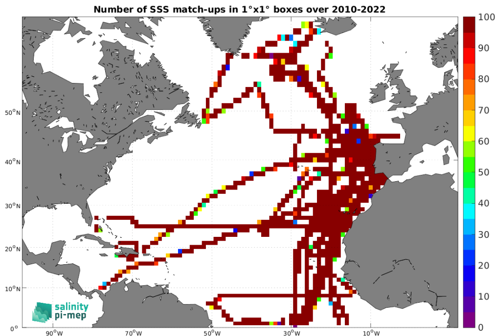
Figure 5: Number of SSS match-ups between TSG (CSIC-UTM) SSS and the SMOS SSS L3 v332 - 9 Days (CATDS-CPDC) SSS product for the North Atlantic Ocean Pi-MEP region over 1^\circ \times 1^\circ boxes and for the full satellite product period.
