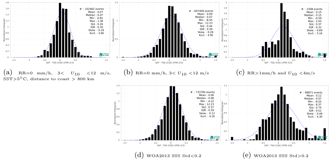
Figure 15: Normalized histogram of \Delta SSS (SMOS SSS L3 v332 - 9 Days (CATDS-CPDC) - TSG (CSIC-UTM)) for 5 different subdatasets corresponding to: RR=0 mm/h, 3 < U_{10} < 12 m/s, SST >5^{\circ} C, distance to coast > 800 km (a), RR=0 mm/h, 3 < U_{10} < 12 m/s (b), RR >1 mm/h and U_{10} < 4 m/s (c), WOA2013 SSS Std <0.2 (d), WOA2013 SSS Std >0.2 (e).
