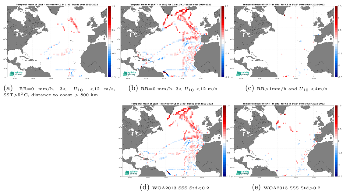
Figure 14: Temporal mean gridded over spatial boxes of size 1^\circ \times 1^\circ of \Delta SSS (SMOS SSS L3 v332 - 9 Days (CATDS-CPDC) - TSG (CSIC-UTM)) for 5 different subdatasets corresponding to:RR=0 mm/h, 3 < U_{10} < 12 m/s, SST >5^\circ\text{C} , distance to coast > 800 km (a), RR=0 mm/h, 3 < U_{10} < 12 m/s (b), RR >1 mm/h and U_{10} < 4 m/s (c), WOA2013 SSS Std <0.2 (d), WOA2013 SSS Std >0.2 (e).
