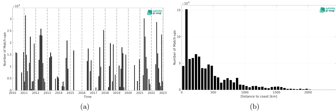
Figure 1: Number of match-ups between TSG (CSIC-UTM) and SMOS SSS L3 v332 - 9 Days (CATDS-CPDC) SSS as a function of time (a) and as function of the distance to coast (b) over the North Atlantic Ocean Pi-MEP region and for the full satellite product period.
