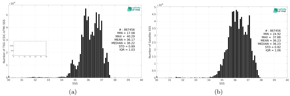
Figure 2: Histograms of SSS from TSG (CSIC-UTM) (a) and SMOS SSS L3 v332 - 9 Days (CATDS-CPDC) (b) considering all match-up pairs per bins of 0.1 over the North Atlantic Ocean Pi-MEP region and for the full satellite product period.
