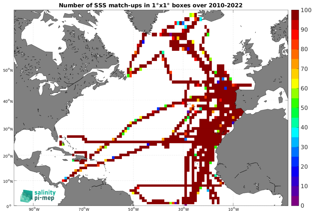
Figure 4: Number of SSS match-ups between TSG (CSIC-UTM) SSS and the SMOS SSS L3 v332 - 9 Days (CATDS-CPDC) SSS product for the North Atlantic Ocean Pi-MEP region over 1^\circ \times 1^\circ boxes and for the full satellite product period.
