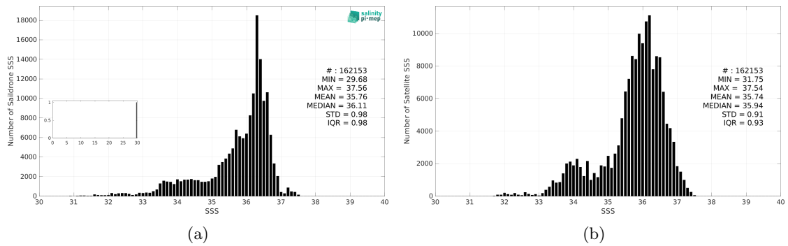
Figure 3: Histograms of SSS from Saildrone (a) and SMOS SSS L3 v332 - 9 Days (CATDS-CPDC) (b) considering all match-up pairs per bins of 0.1 over the North Atlantic Ocean Pi-MEP region and for the full satellite product period.
