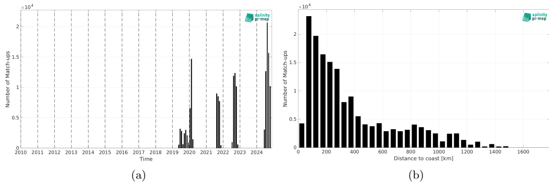
Figure 2: Number of match-ups between Saildrone and SMOS SSS L3 v332 - 9 Days (CATDS-CPDC) SSS as a function of time (a) and as function of the distance to coast (b) over the North Atlantic Ocean Pi-MEP region and for the full satellite product period.
