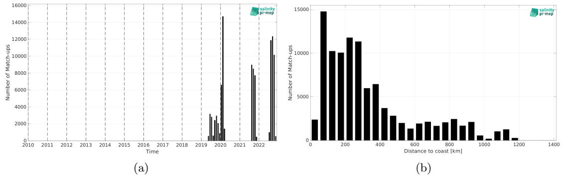
Figure 2: Number of match-ups between Sairdrone and SMOS SSS L3 v332 - 9 Days (CATDS-CPDC) SSS as a function of time (a) and as function of the distance to coast (b) over the North Atlantic Ocean Pi-MEP region and for the full satellite product period.
