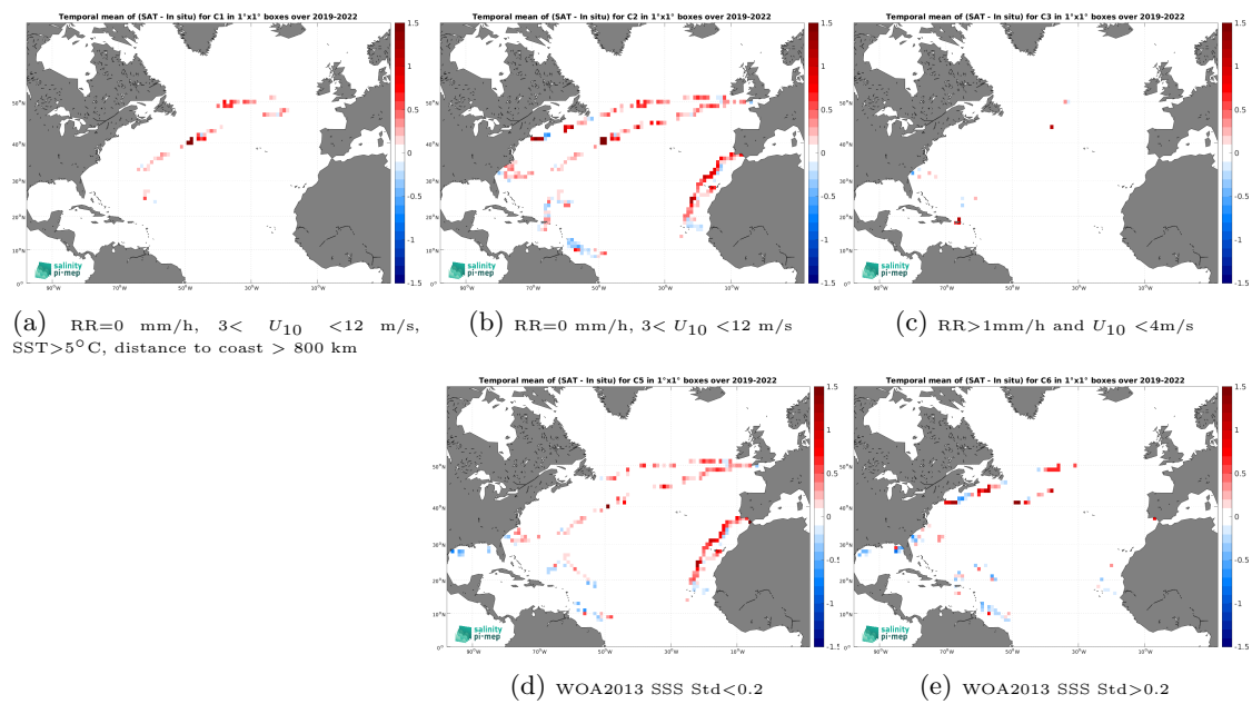
Figure 14: Temporal mean gridded over spatial boxes of size 1^\circ \times 1^\circ of \Delta SSS (SMOS SSS L3 v332 - 9 Days (CATDS-CPDC) - Saildrone) for 5 different subdatasets corresponding to:RR=0 mm/h, 3 < U_{10} < 12 m/s, SST >5^\circ C, distance to coast > 800 km (a), RR=0 mm/h, 3 < U_{10} < 12 m/s (b), RR >1 mm/h and U_{10} < 4 m/s (c), WOA2013 SSS Std <0.2 (d), WOA2013 SSS Std >0.2 (e).
