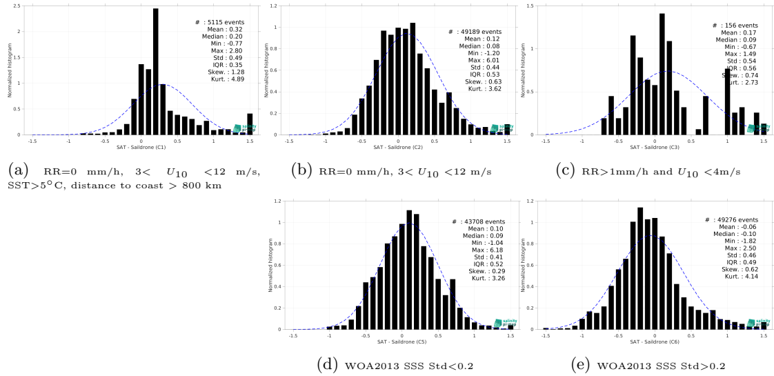
Figure 15: Normalized histogram of \Delta SSS (SMOS SSS L3 v332 - 9 Days (CATDS-CPDC) - Saldrone) for 5 different subdatasets corresponding to: RR=0 mm/h, 3 < U_{10} < 12 m/s, SST>5°C, distance to coast > 800 km (a), RR=0 mm/h, 3 < U_{10} < 12 m/s (b), RR>1mm/h and U_{10} < 4 m/s (c), WOA2013 SSS Std<0.2 (d), WOA2013 SSS Std>0.2 (e).
