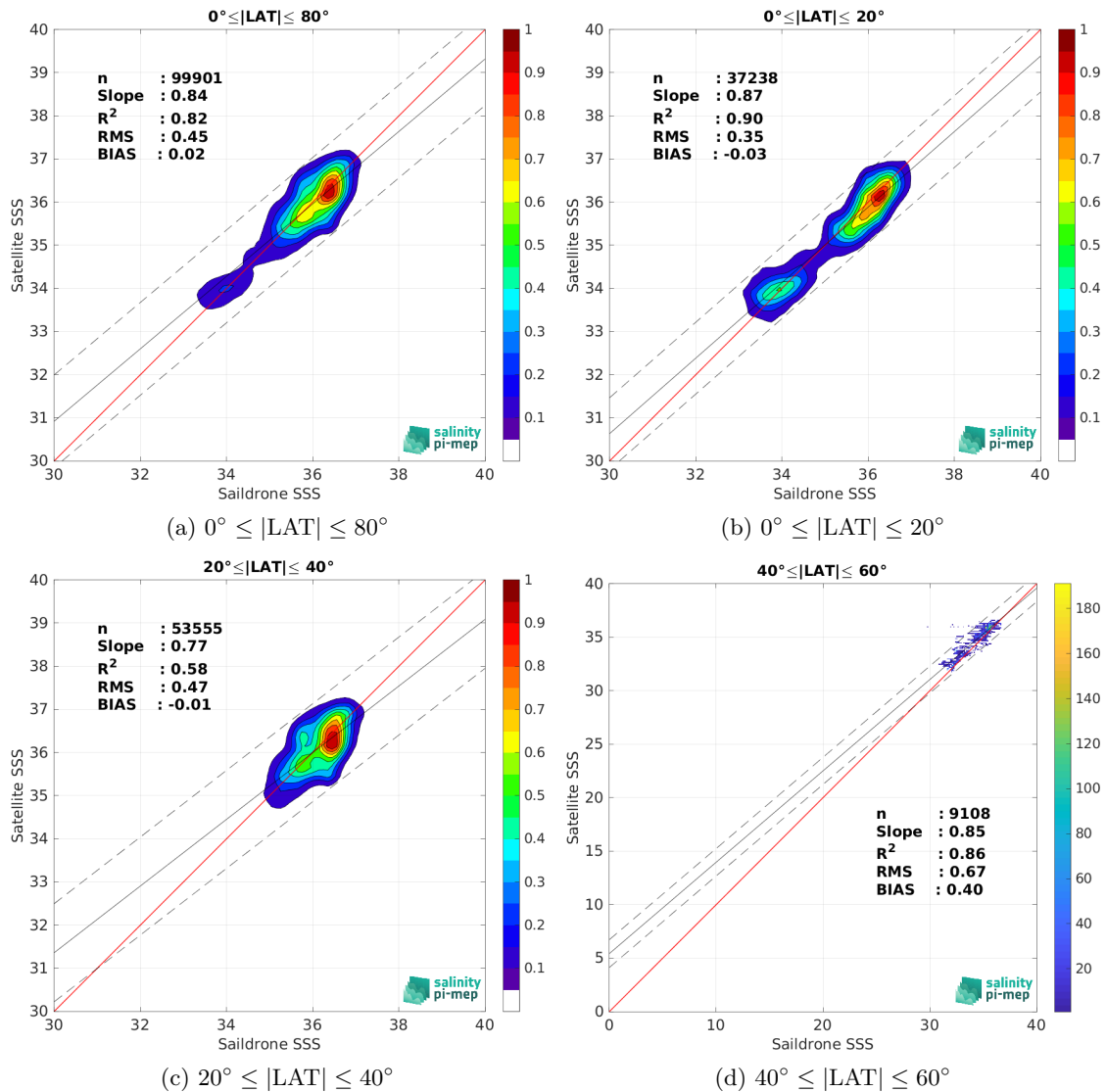
Figure 10: Contour maps of the concentration of SMOS SSS L3 v332 - 9 Days (CATDS-CPDC) SSS (y-axis) versus Sailability SSS (x-axis) at match-up pairs for different latitude bands. For each plot, the red line shows x=y . The black thin and dashed lines indicate a linear fit through the data cloud and the \pm 95\% confidence levels, respectively. The number match-up pairs n , the slope and R^2 coefficient of the linear fit, the root mean square (RMS) and the mean bias between satellite and in situ data are indicated for each latitude band in each plots.
