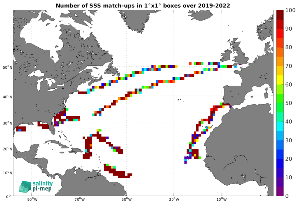
Figure 5: Number of SSS match-ups between Saildrone SSS and the SMOS SSS L3 v332 - 9 Days (CATDS-CPDC) SSS product for the North Atlantic Ocean Pi-MEP region over 1^\circ \times 1^\circ boxes and for the full satellite product period.
