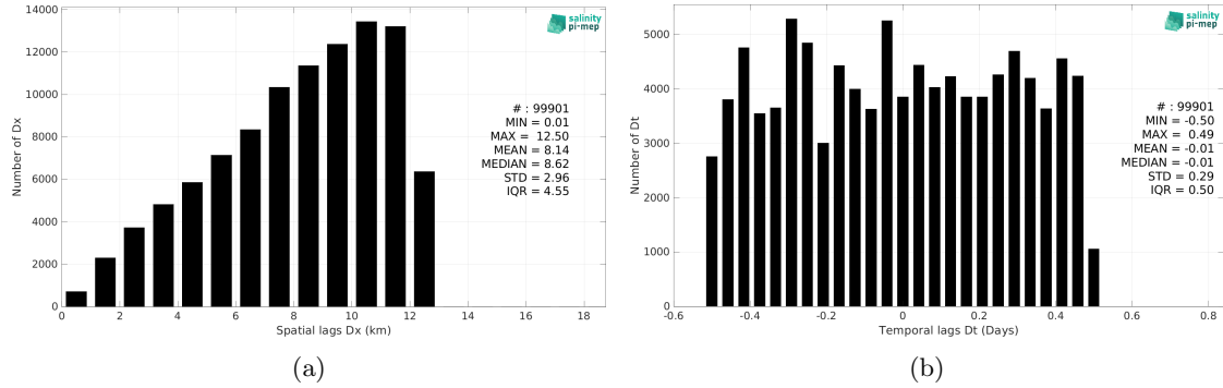
Figure 6: Histograms of the spatial (a) and temporal (b) lags between the location/time of the Sairdrone measurement and the date of the corresponding SMOS SSS L3 v332 - 9 Days (CATDS-CPDC) SSS pixel.
