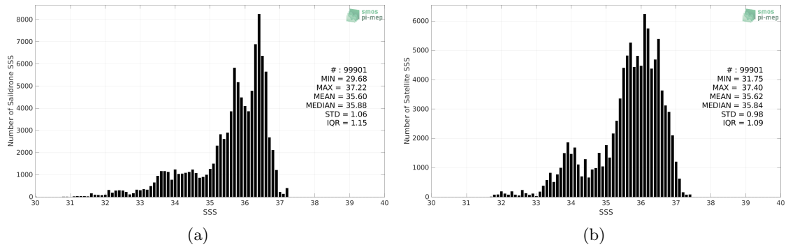
Figure 2: Histograms of SSS from Sailldrone (a) and SMOS SSS L3 v332 - 9 Days (CATDS-CPDC) (b) considering all match-up pairs per bins of 0.1 over the North Atlantic Ocean Pi-MEP region and for the full satellite product period.
