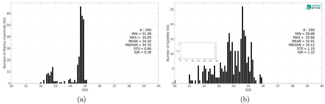
Figure 3: Histograms of SSS from Marine mammals (a) and SMOS SSS L3 v332 - 9 Days (CATDS-CPDC) (b) considering all match-up pairs per bins of 0.1 over the North Atlantic Ocean Pi-MEP region and for the full satellite product period.
