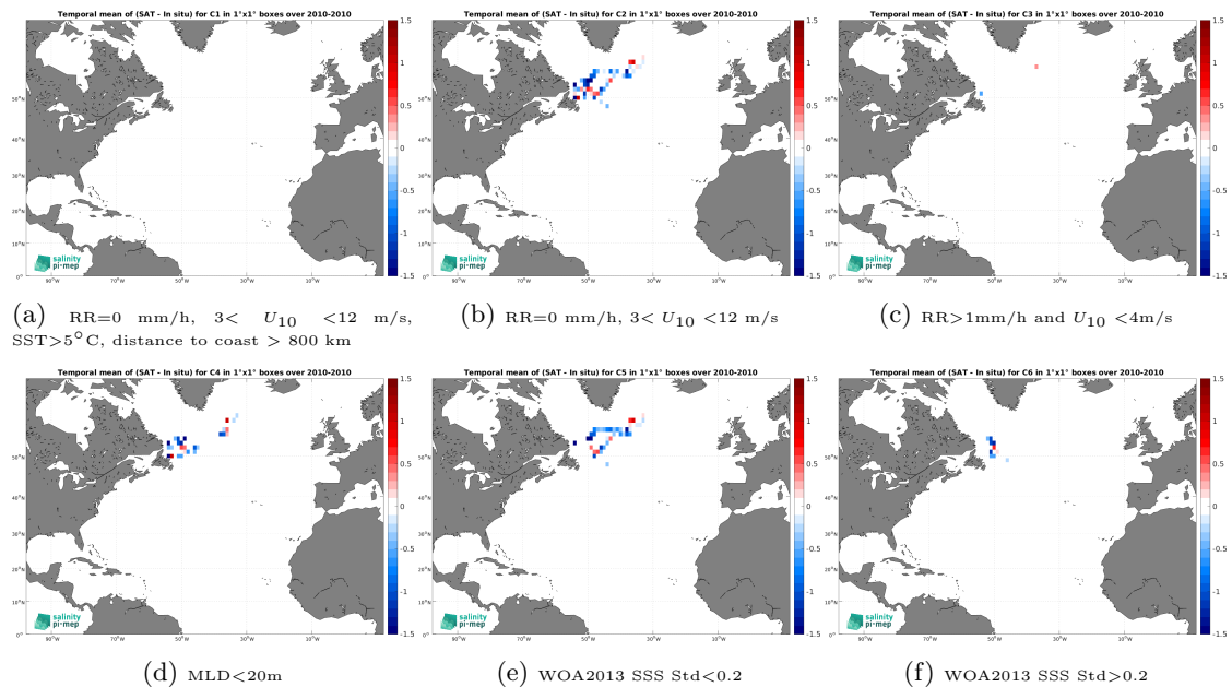
Figure 14: Temporal mean gridded over spatial boxes of size 1^\circ \times 1^\circ of \Delta SSS (SMOS SSS L3 v332 - 9 Days (CATDS-CPDC) - Marine mammals) for 6 different subdatasets corresponding to:RR=0 mm/h, 3 < U_{10} < 12 m/s, SST > 5^\circ\text{C} , distance to coast > 800 km (a), RR=0 mm/h, 3 < U_{10} < 12 m/s (b), RR > 1 mm/h and U_{10} < 4 m/s (c),MLD < 20 m (d),WOA2013 SSS Std < 0.2 (e),WOA2013 SSS Std > 0.2 (f).
