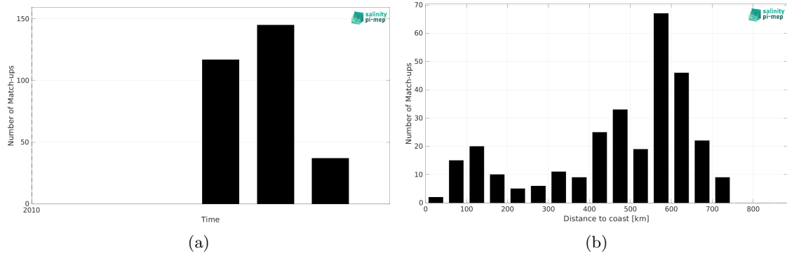
Figure 2: Number of match-ups between Marine mammals and SMOS SSS L3 v332 - 9 Days (CATDS-CPDC) SSS as a function of time (a) and as function of the distance to coast (b) over the North Atlantic Ocean Pi-MEP region and for the full satellite product period.
