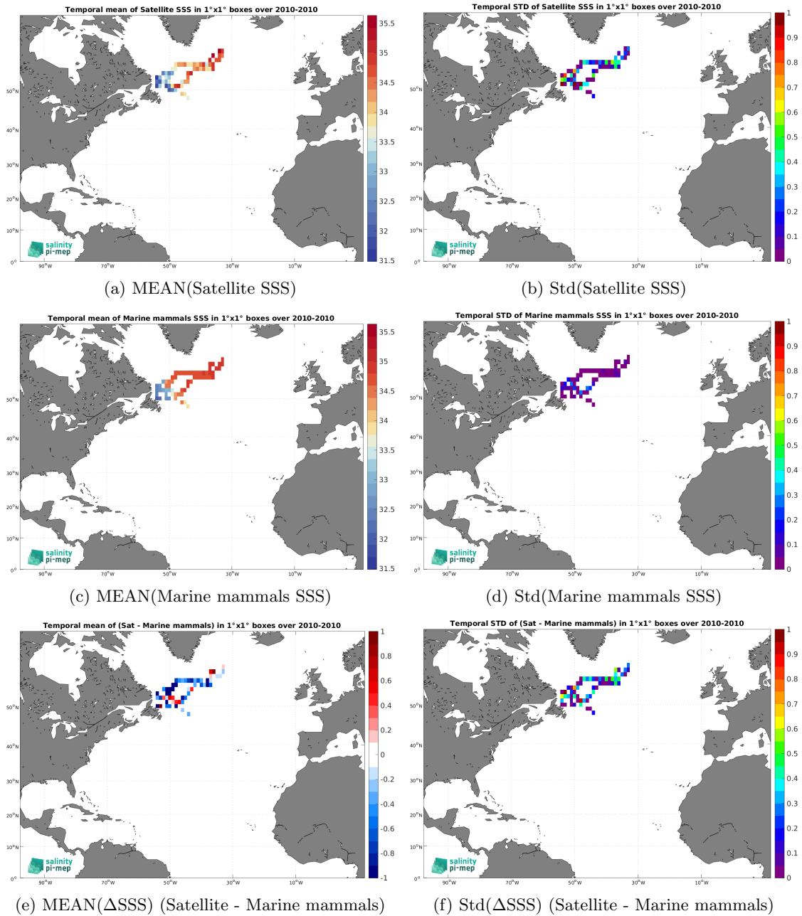
Figure 7: Temporal mean (left) and Std (right) of SSS from SMOS SSS L3 v332 - 9 Days (CATDS-CPDC) (top), Marine mammals (middle), and of \Delta SSS (Satellite - Marine mammals). Only match-up pairs are used to generate these maps.
