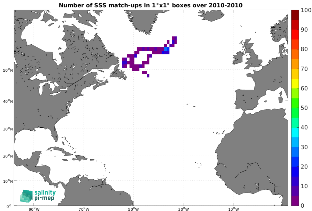
Figure 5: Number of SSS match-ups between Marine mammals SSS and the SMOS SSS L3 v332 - 9 Days (CATDS-CPDC) SSS product for the North Atlantic Ocean Pi-MEP region over 1^\circ \times 1^\circ boxes and for the full satellite product period.
