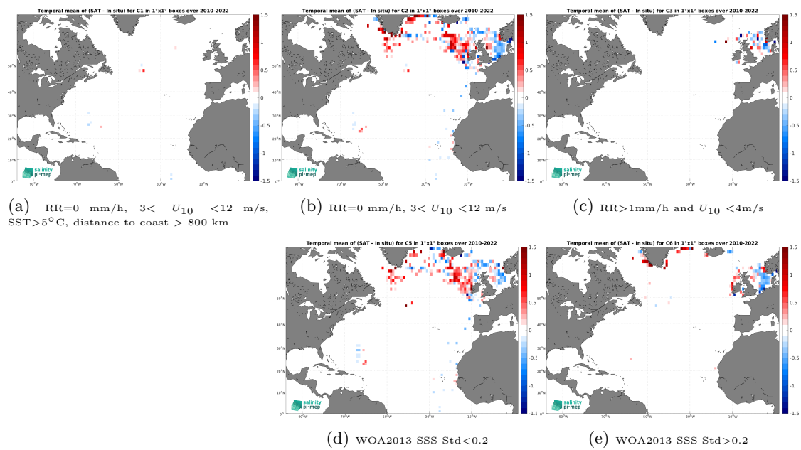
Figure 14: Temporal mean gridded over spatial boxes of size 1^\circ \times 1^\circ of \Delta\text{SSS} (SMOS SSS L3 v332 - 9 Days (CATDS-CPDC) - ICES) for 5 different subdatasets corresponding to:RR=0 mm/h, 3 < U_{10} < 12 m/s, SST >5^\circ\text{C} , distance to coast > 800 km (a), RR=0 mm/h, 3 < U_{10} < 12 m/s (b), RR >1 mm/h and U_{10} < 4 m/s (c), WOA2013 SSS Std <0.2 (d), WOA2013 SSS Std >0.2 (e).
